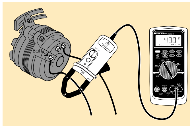
Figure 2. Verifying a good alternator
