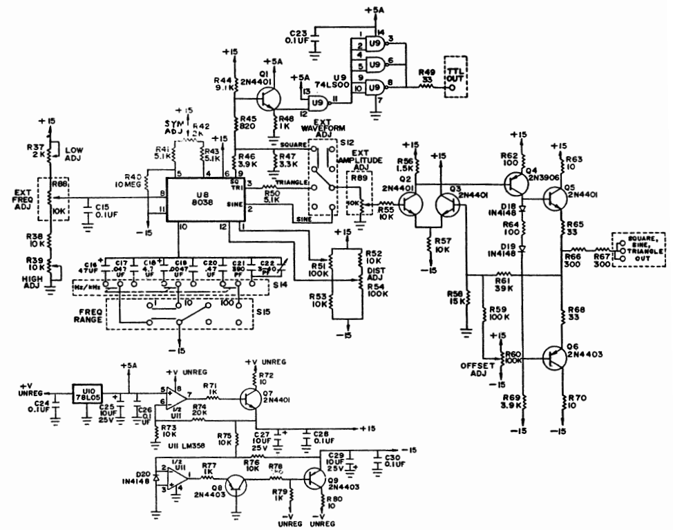
FIGURE 7. PB-503 Circuit Schematic
