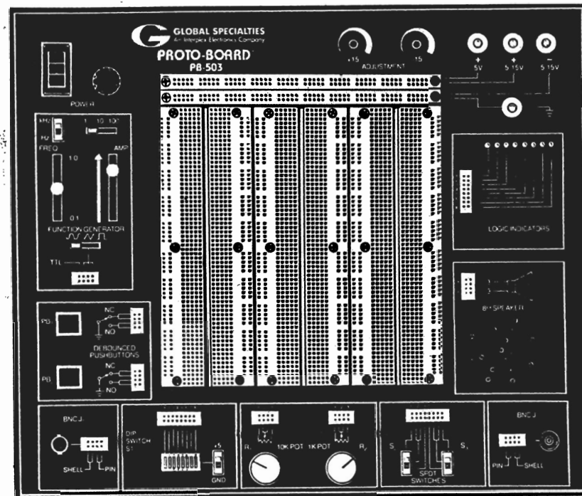
FIGURE 1. PB-503 panel layout
