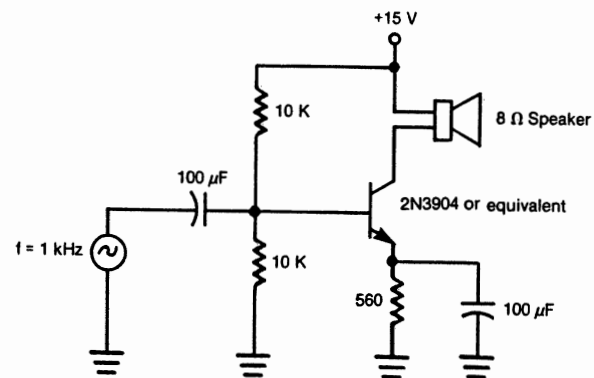
FIGURE 3. One-transistor audio amplifier
