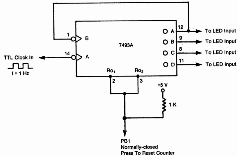
FIGURE 5. 4-Bit resettable binary counter
