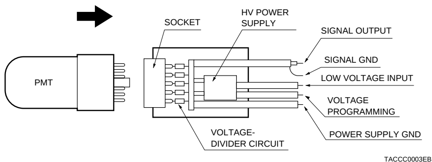
Figure 1-12: DP type socket assembly
