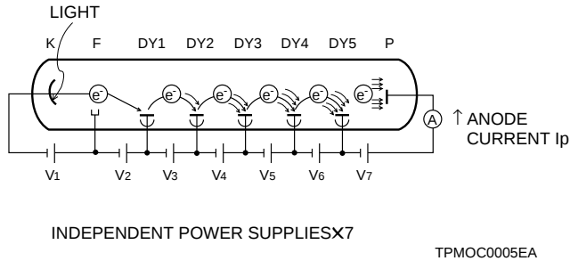
Figure 7-1: Schematic diagram of photomultiplier tube operation
