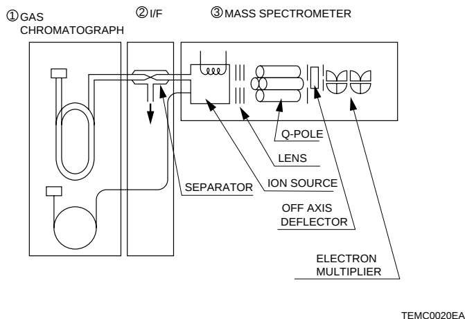
Figure 9-40: Schematic drawing of a gas chromatograph mass spectrometer.
