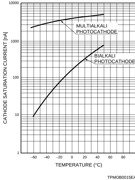
Figure 8-2: Cathode saturation current vs. temperature
