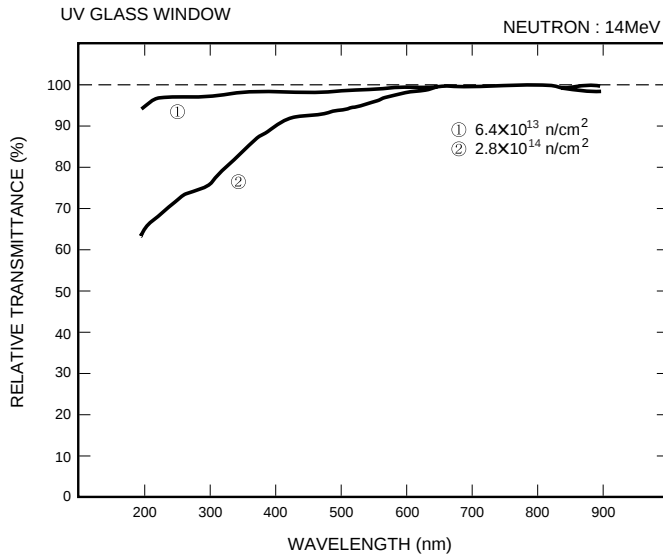
Figure 8-12 (b): Transmittance variations of UV glass window when irradiated by neutrons
