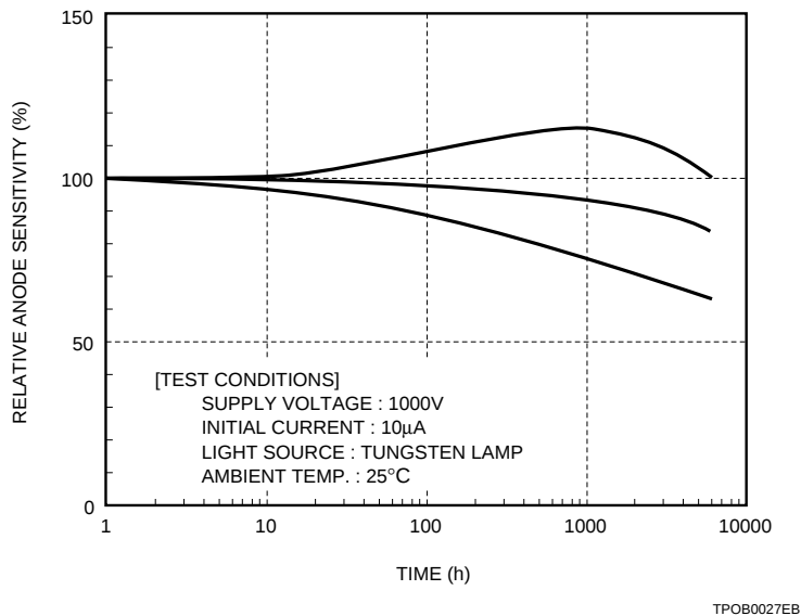
Figure 8-19: Typical time stability of photomultiplier tubes
