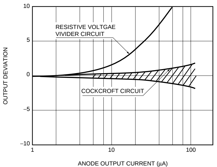
Figure 7-16: Output linearity
