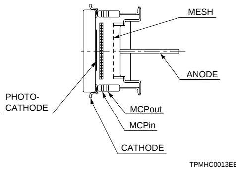
Figure 4-14: Structure of the R7024
