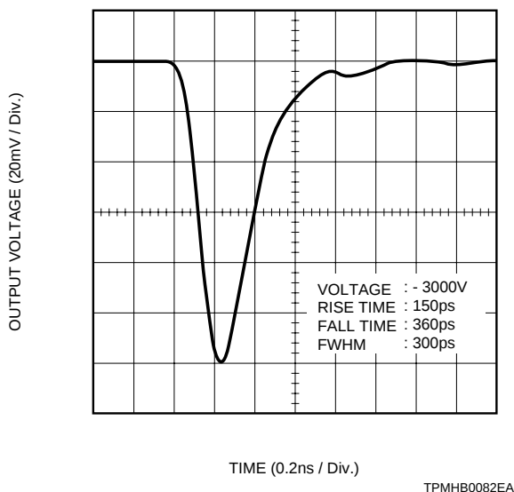
Figure 4-11: Pulse response waveform of MCP-PMT (R3809U-50)
