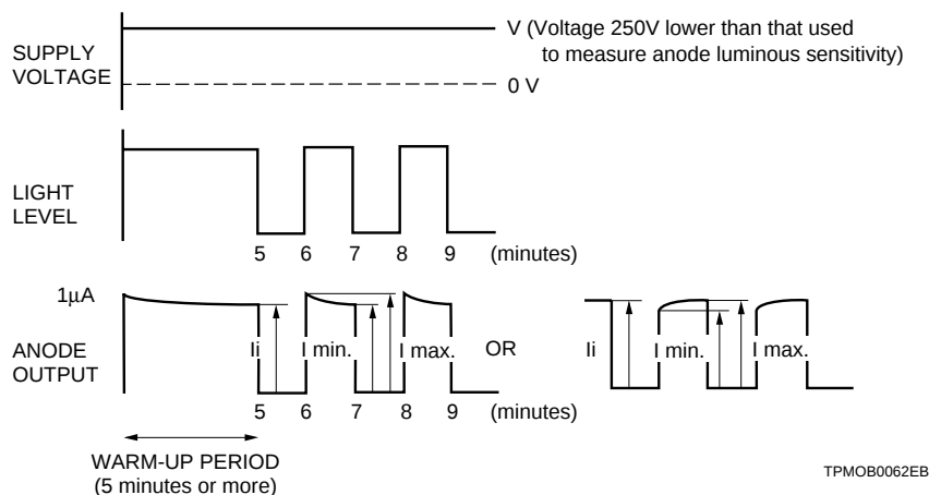
Figure 3-34: Light hysteresis
