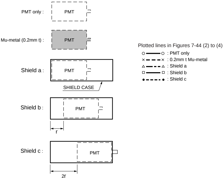
Figure 7-44 (1): Photomultiplier tube shield conditions for magnetic characteristic measurements
