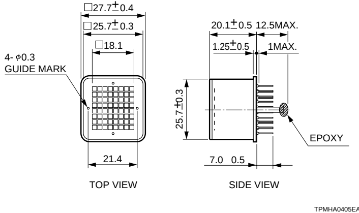
Figure 6-8: R5900-00-M64 external dimensions
