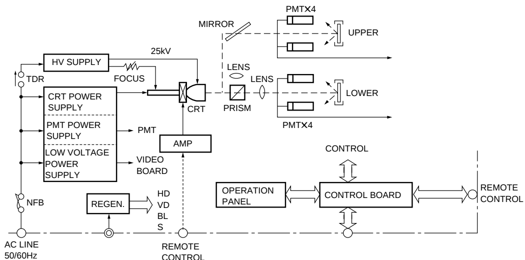
Figure 9-60: Block diagram of a flying spot scanner
