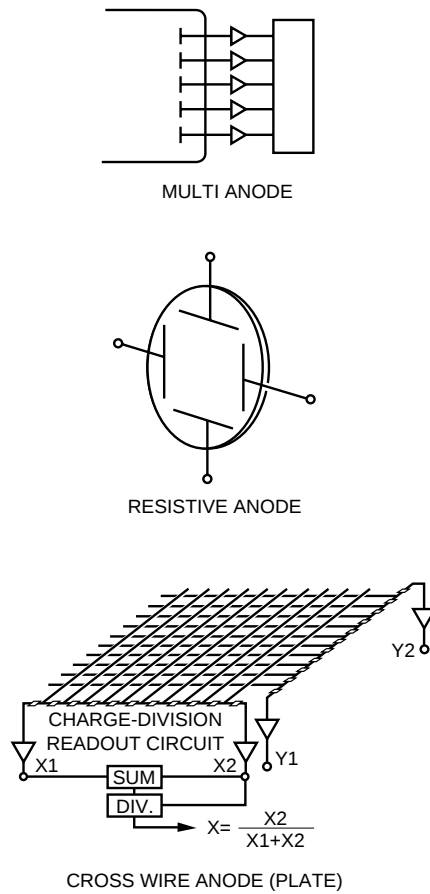
Figure 6-1: Anode output readout methods for position-sensitive photomultiplier tube
