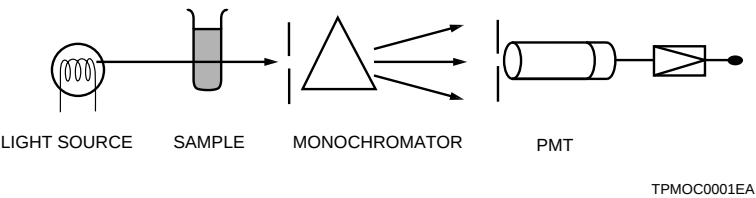
Figure 1-6: Atomic absorption application
