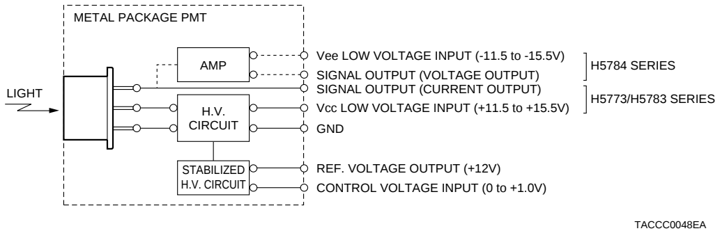
Figure 1-13: Structure of an integral power supply module
