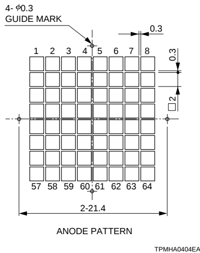
Figure 6-9: R5900-00-M64 anode pattern
