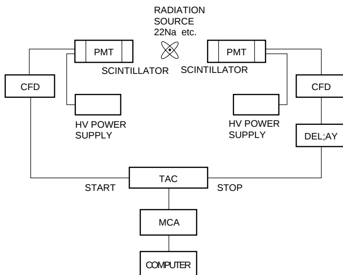
Figure 3-20: Block diagram for CRT measurement
