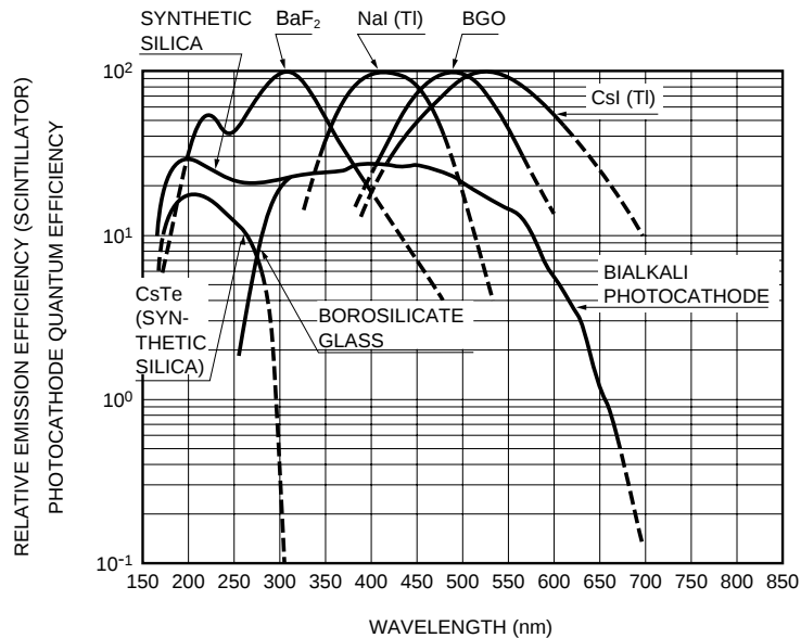
Figure 3-58: Photocathode quantum efficiency and emission spectra of major scintillators
