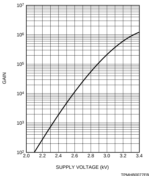
Figure 4-5: Typical gain of an MCP-PMT (using a two-stage MCP of 6μm channel diameter)
