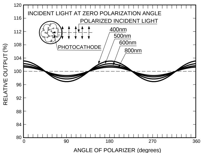
Figure 3-44: Typical polarization-light dependence of a side-on photomultiplier tube
