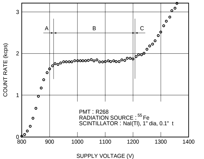
Figure 3-66: Plateau characteristic (a)
