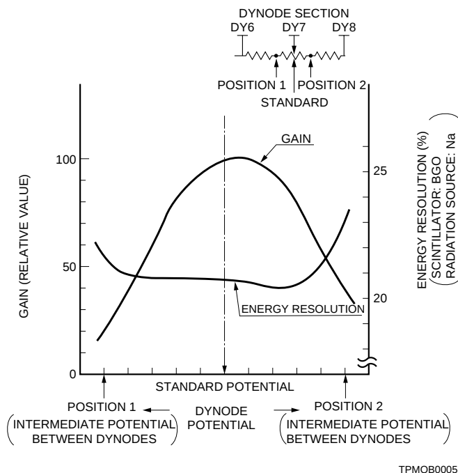
Figure 7-19: Gain variation and energy resolution as a function of dynode potential
