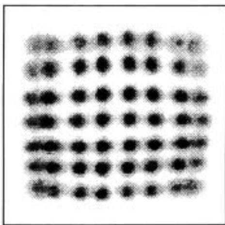
Position data after calculation when gamma-rays at 511keV were incident on the 8x7 BGO array (2.8mmX2.8mmX30mm)
