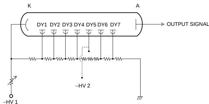
Figure 7-18: Output control circuits
