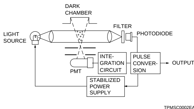
Figure 9-45: Block diagram of a dust counter using light scattering
