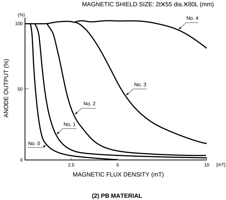
Figure 7-41: Magnetic characteristics of a photomultiplier tube used with magnetic shield case (2)
