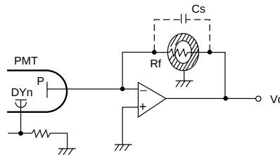
Figure 7-29: Canceling the stray capacitance C_s
