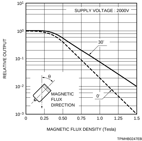
Figure 8-6 (2): Magnetic characteristics of photomultiplier tubes for highly magnetic fields
