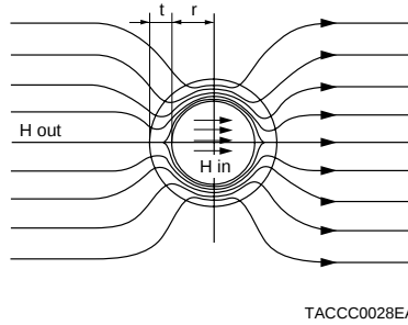
Figure 7-37: Shielding effect of a magnetic shield case
