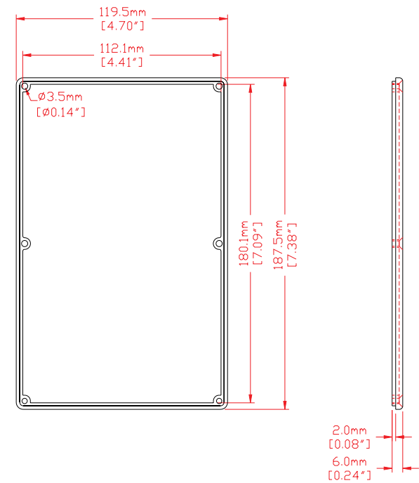
VIEW INSIDE LID
