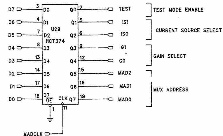
MUX CONTROL LATCHES
