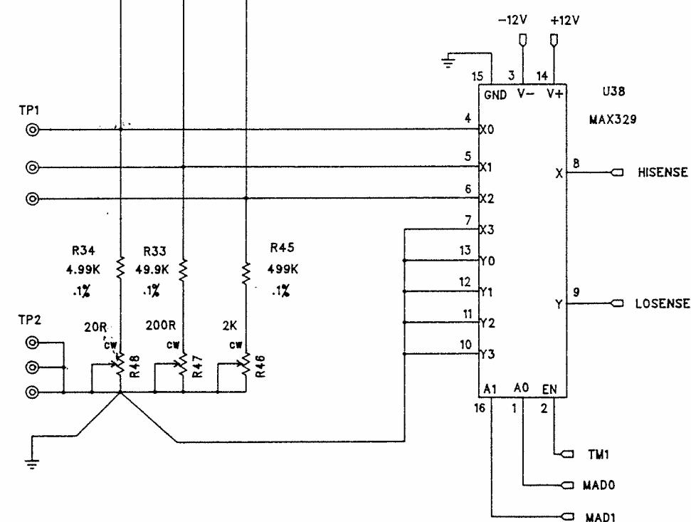
TEST MULTIPLEXERS
