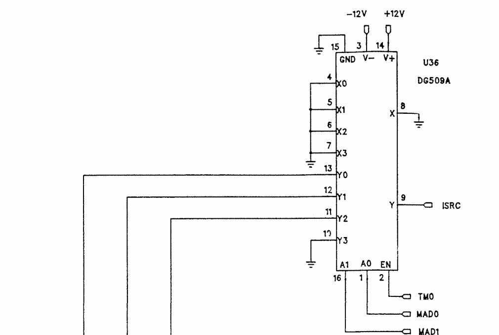
TEST MULTIPLEXERS
