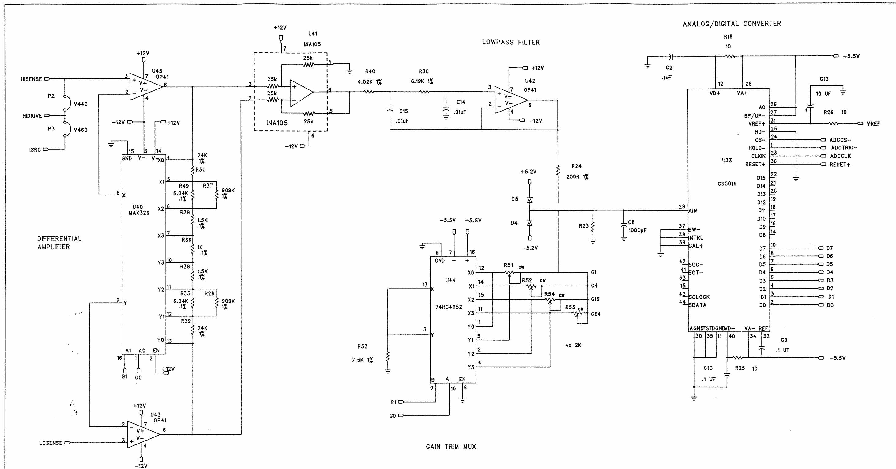
DIFFAMP AND ADC
