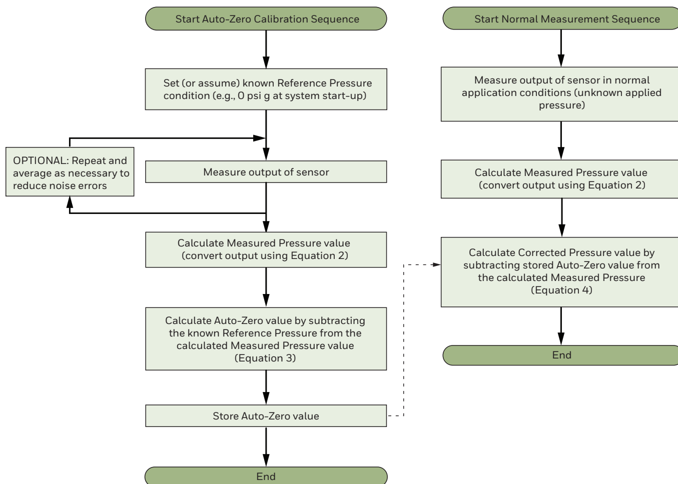
Figure 4. How to Implement Auto-Zero Calibration and Correction
