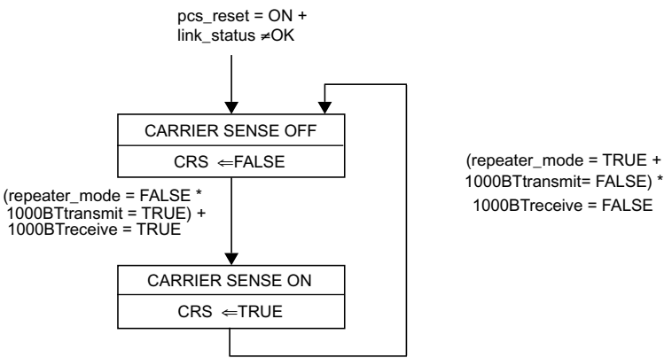
Figure 40–11 — PCS Carrier Sense state diagram
