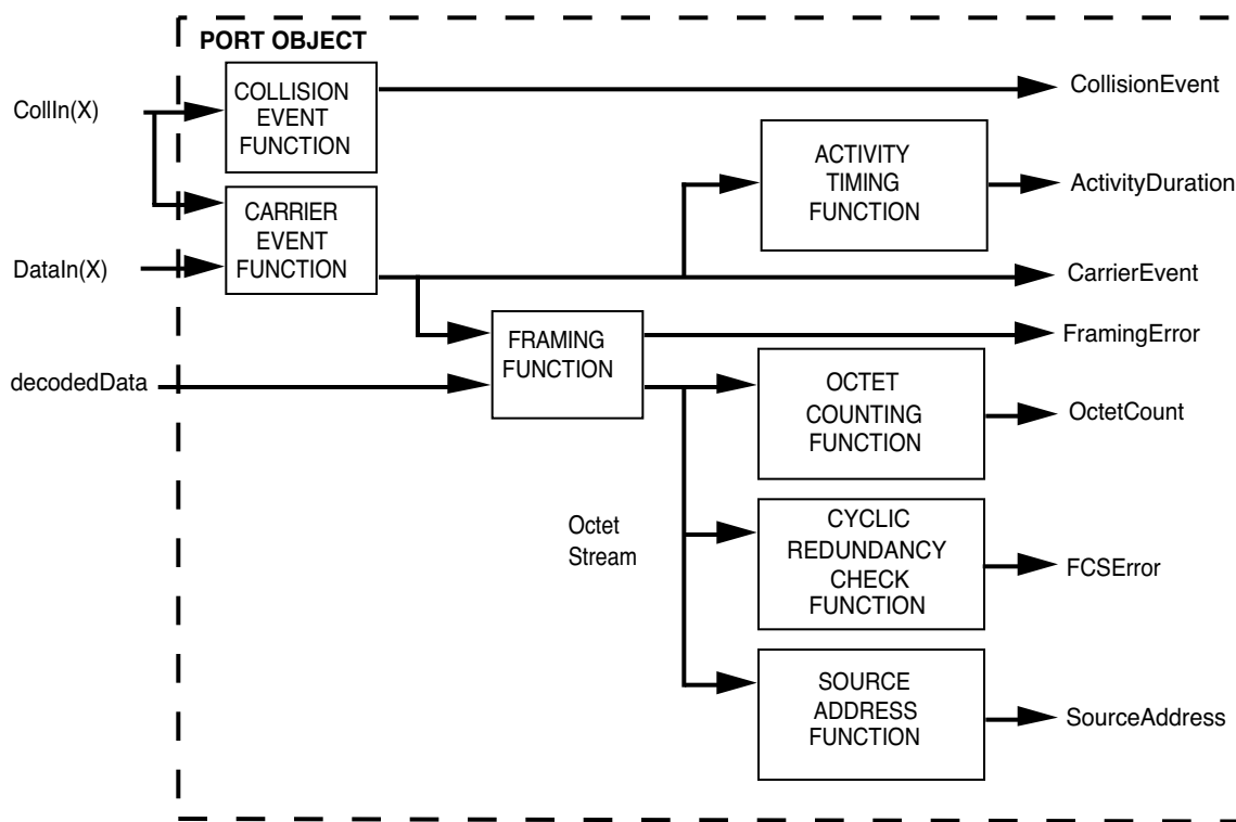
Figure 19-2—Functions relationship
