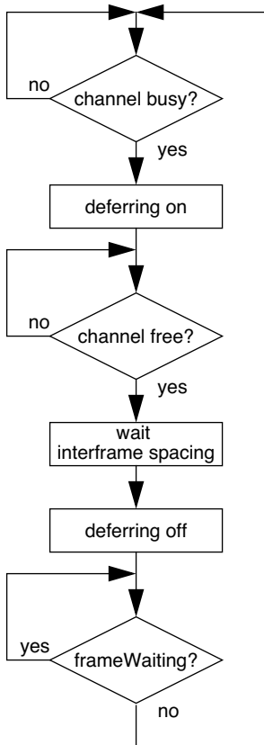
Deference process
