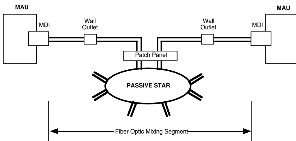
b) Example fiber optic mixing segment, 10BASE-FP
