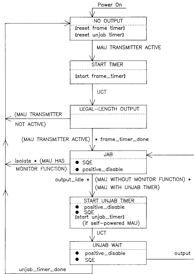
Figure 8–4—Jabber function
