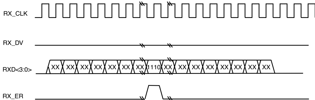
Figure 22–8—False Carrier indication
