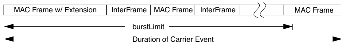
Figure 4–1 – Frame bursting
