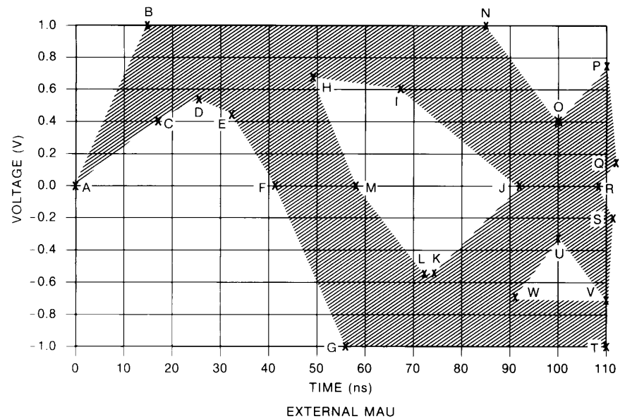
Figure 14-9—Voltage template
