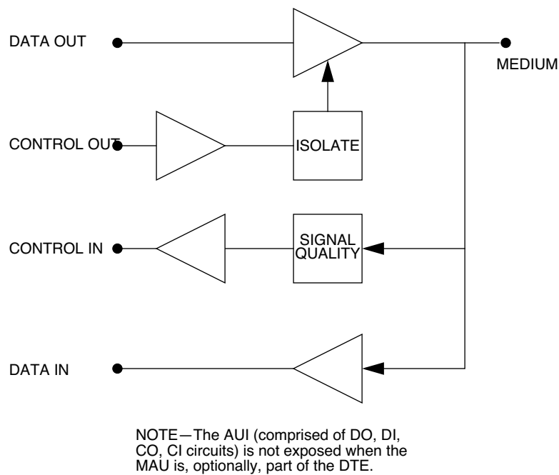
Figure 7-2—Generalized MAU model
