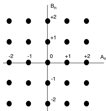
Figure 32–3—PAM5×5 symbol constellation
