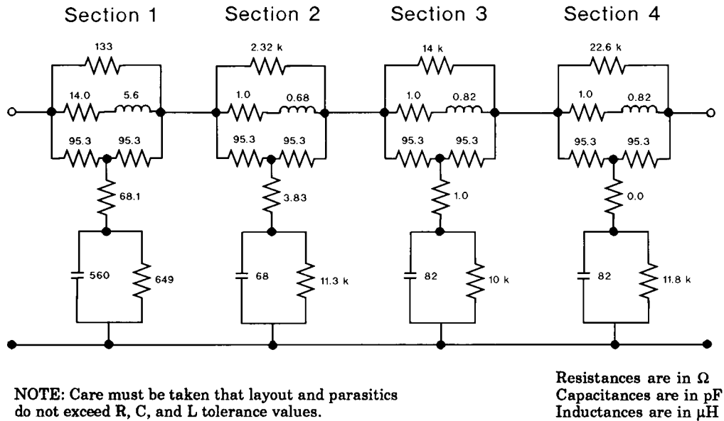
Figure 14-7—Twisted-pair model
