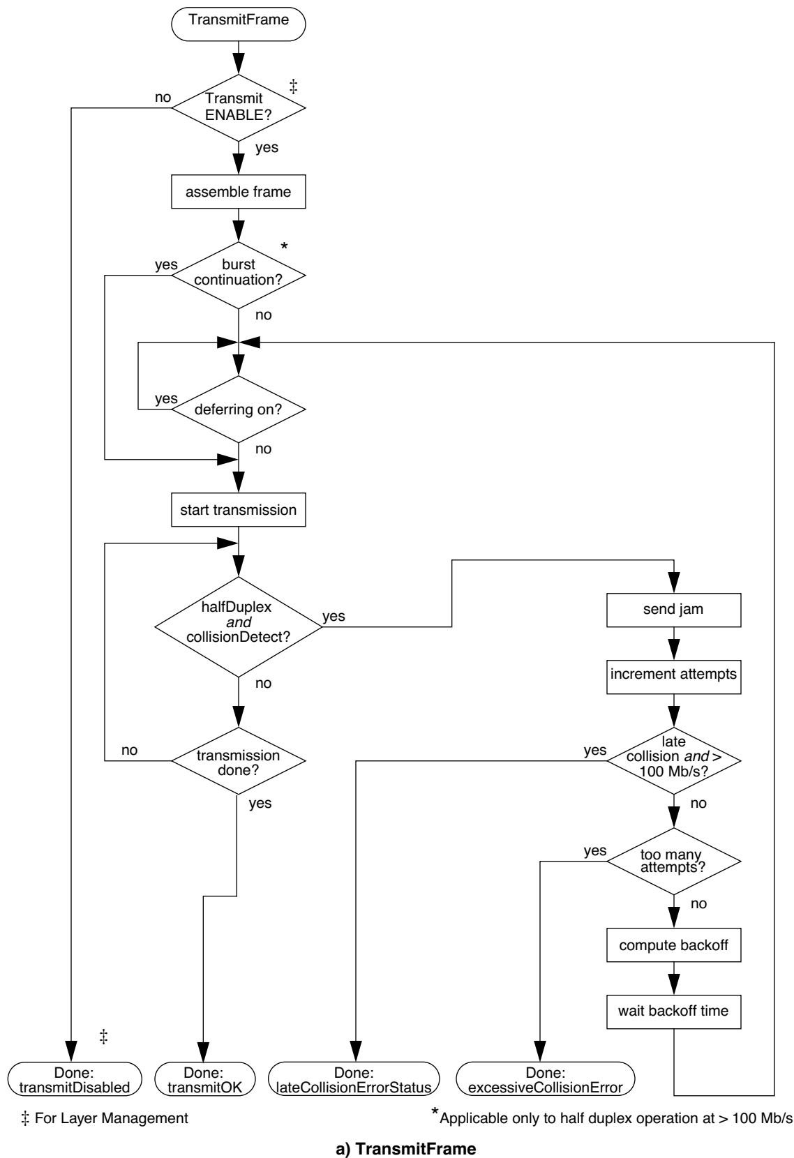
Figure 4–4a—Control flow summary
