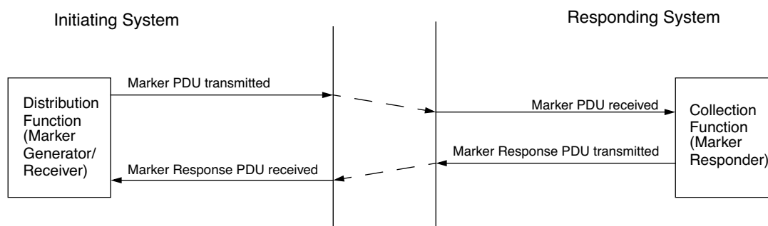
Figure 43–17—Marker protocol time sequence diagram
