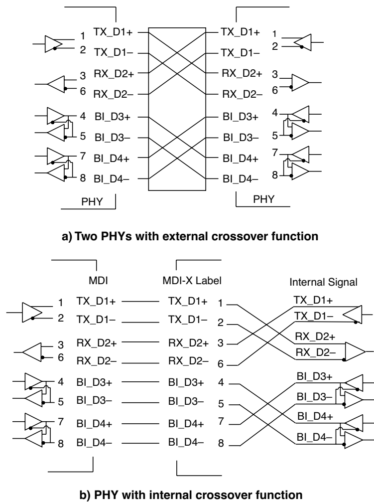
Figure 23–28—Crossover function
