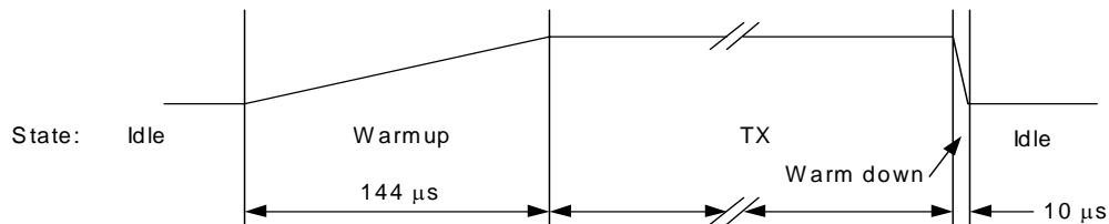
Figure 3-10. TX Timing Profile
