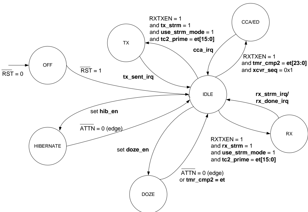
Figure 6-4. State Diagram for Stream Mode With TC2_Prime Enabled State (tmr_trig_en = 1)
