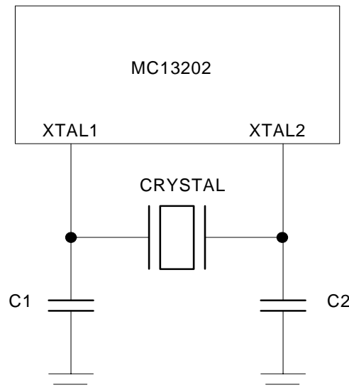
Figure 9-1. Crystal oscillator circuit
