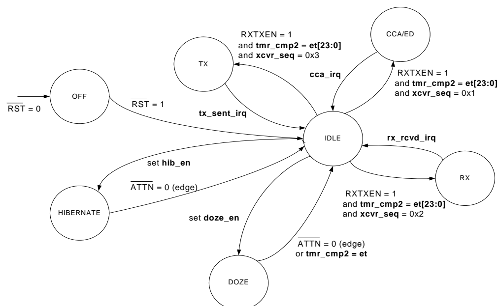
Figure 6-2. State Diagram for Packet Mode With Tmr_Cmp2 Enabled States (tmr_trig_en = 1)
