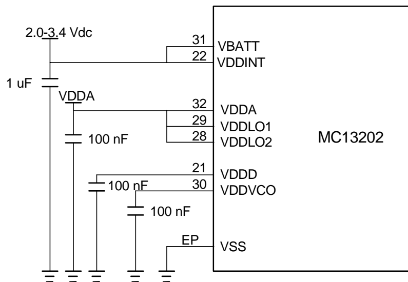
Figure 3-1. MC13202 Power Supply Connections
