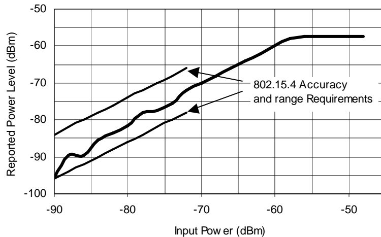
Figure 6-6. CCA Reported Power Level vs. Input Power
