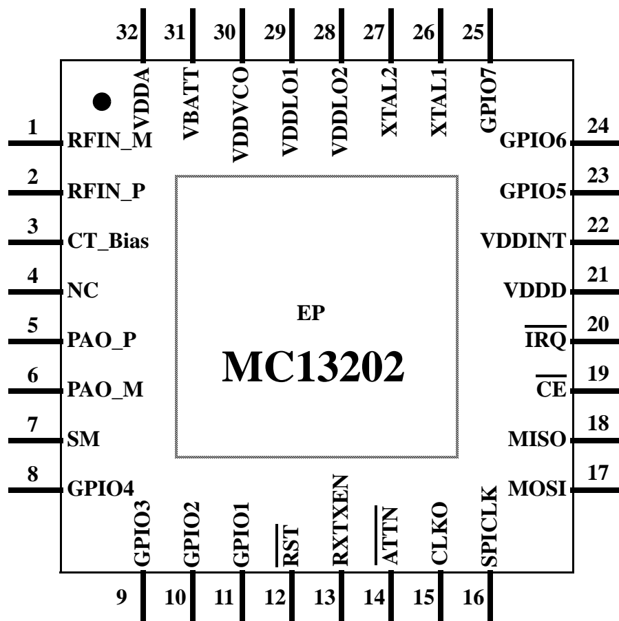
Figure 2-1. MC13202 Pinout
