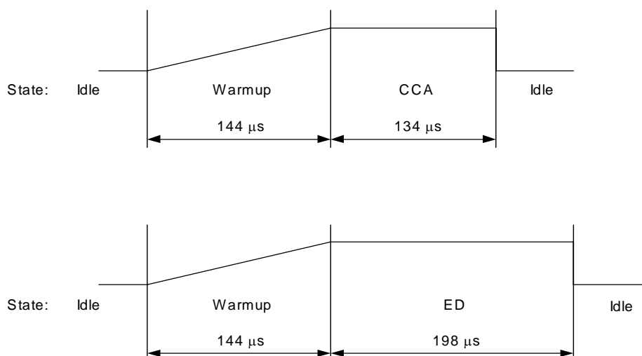
Figure 3-8. CCA and ED Timing Profiles
