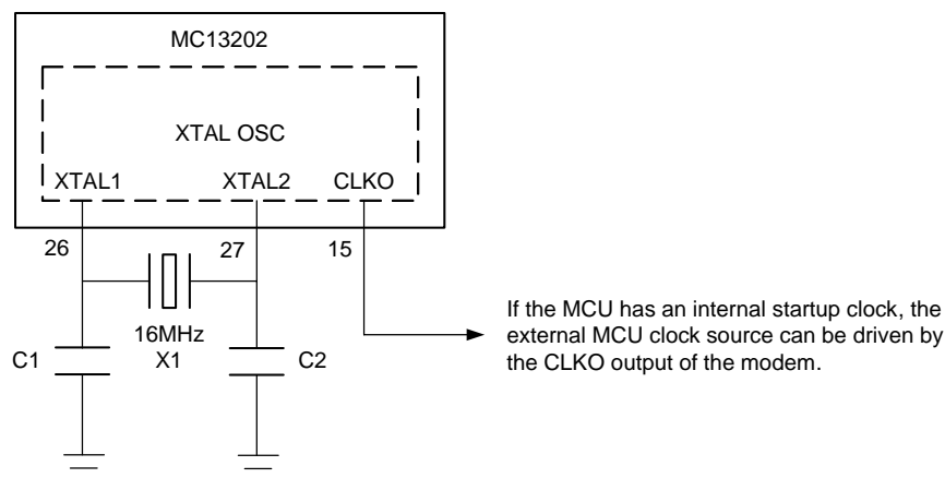
Figure 3-2. MC13202 Oscillator and External Clock Connections
