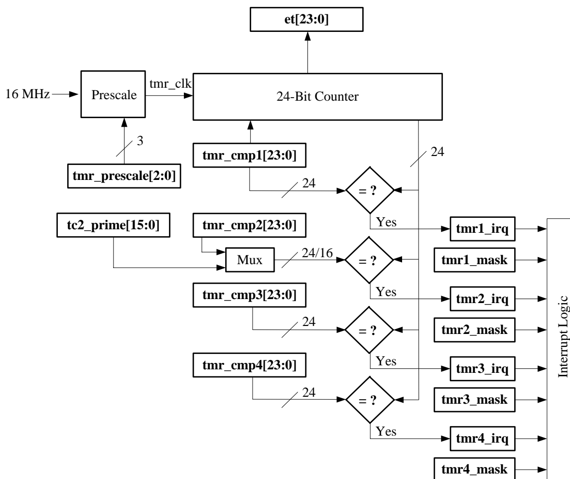
Figure 7-1. Event Timer Block Diagram
