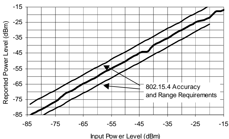
Figure 6-7. ED and LQI Reported Power vs. Input Power
