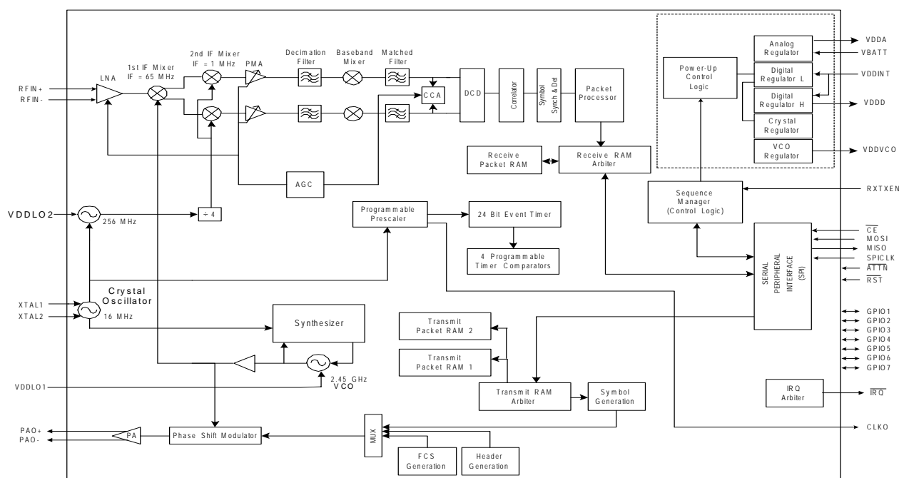
Figure 1-1. MC13202 Simplified Block Diagram
