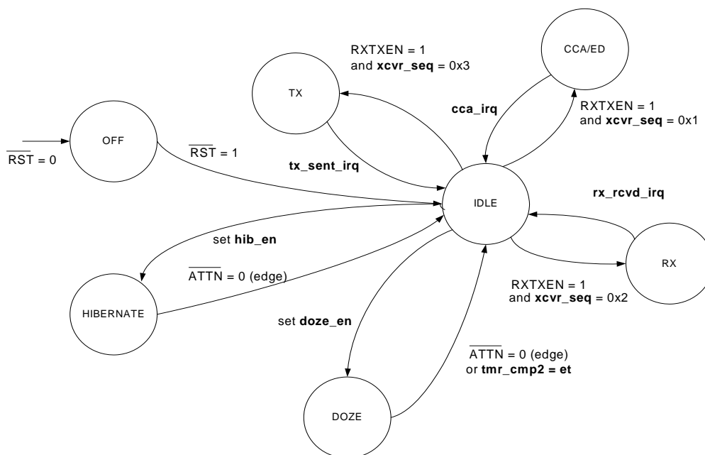
Figure 6-1. State Diagram for Packet Mode Without Timer Enabled States
