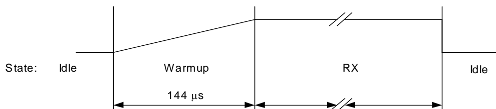
Figure 3-9. RX Timing Profile
