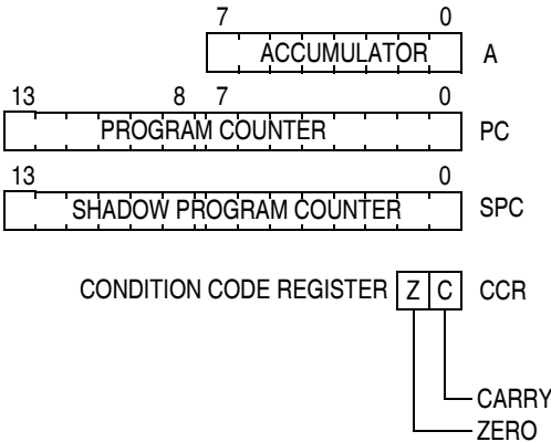
Figure 8-1. CPU Registers
