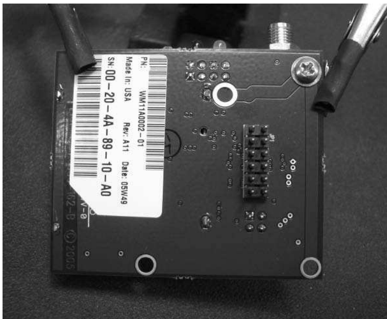
FIGURE 12-3: Underside of WiMicro with hacker-friendly 0.1" header pins
