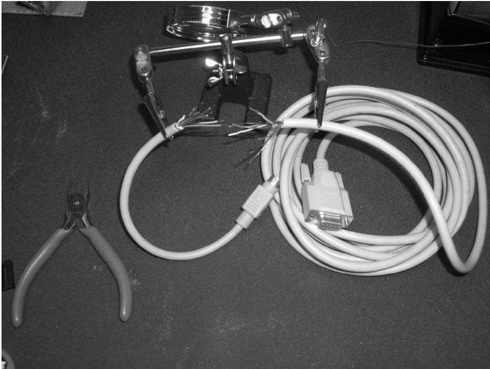
FIGURE 3-8: Mini DIN 8 and DB-9 cables in the third-hand tool, stripped and tinned for the circuit
