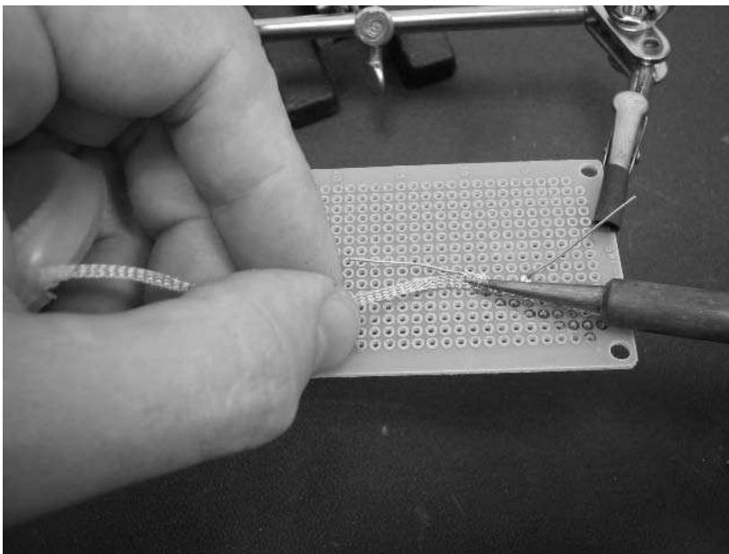
FIGURE A-13: Clean and ready to be resoldered
