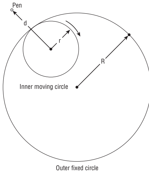
FIGURE 9-10: Spirograph diagram
