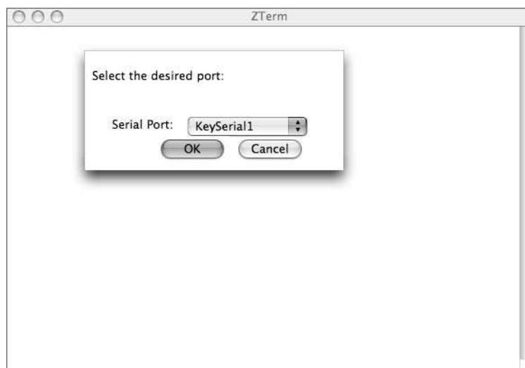
FIGURE 3-15: ZTerm startup
