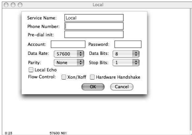
FIGURE 3-16: ZTerm configuration
