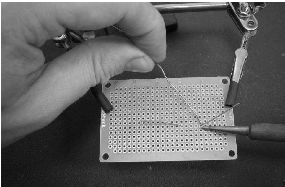
FIGURE A-8: The soldering component, iron on one side, solder on the other
