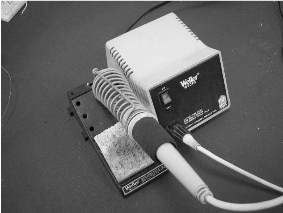
FIGURE A-1: Weller soldering iron with holder and cleaning sponge
