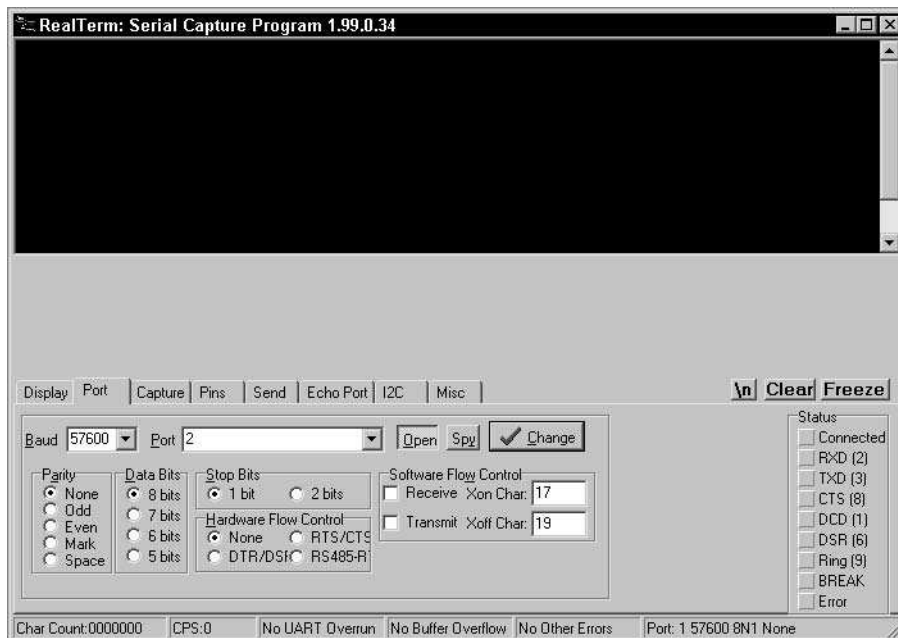
FIGURE 3-18: RealTerm configuration
