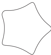
FIGURE 9-10: Spirograph diagram
