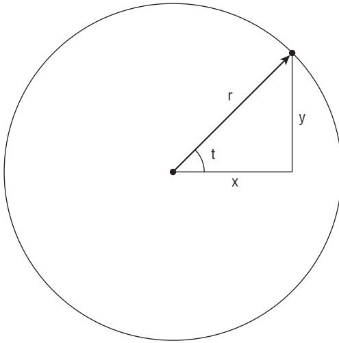
FIGURE 9-12: Circle parameterized
