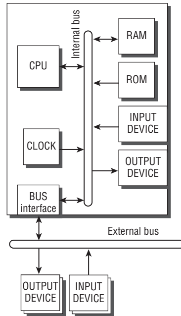
FIGURE 13-1: Typical computer architecture vs. microcontroller architecture
