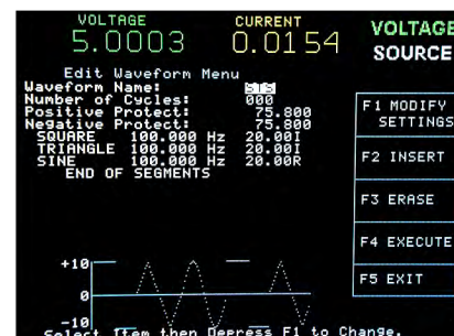
Complex Sine Waveform
