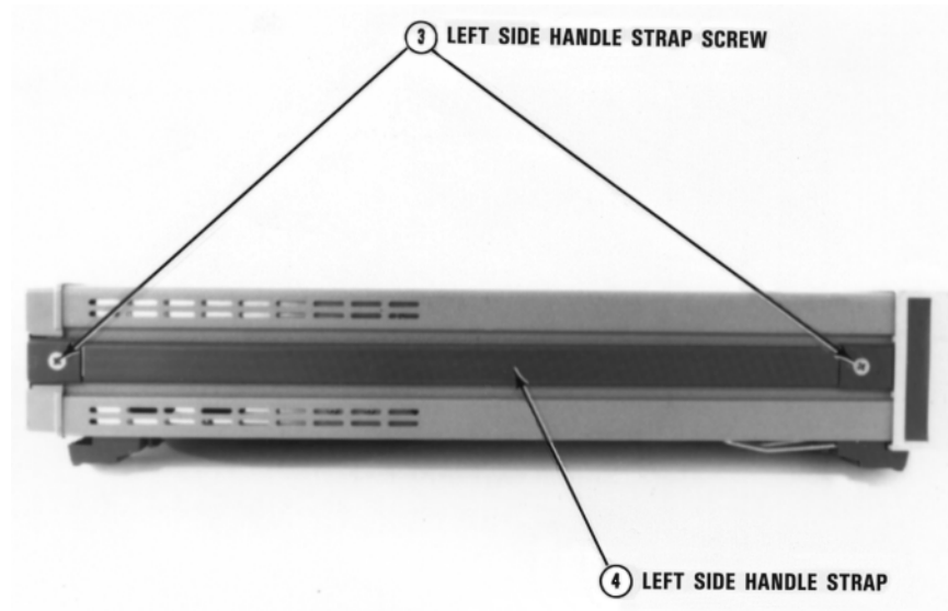
Figure 36. 3458 Left side
