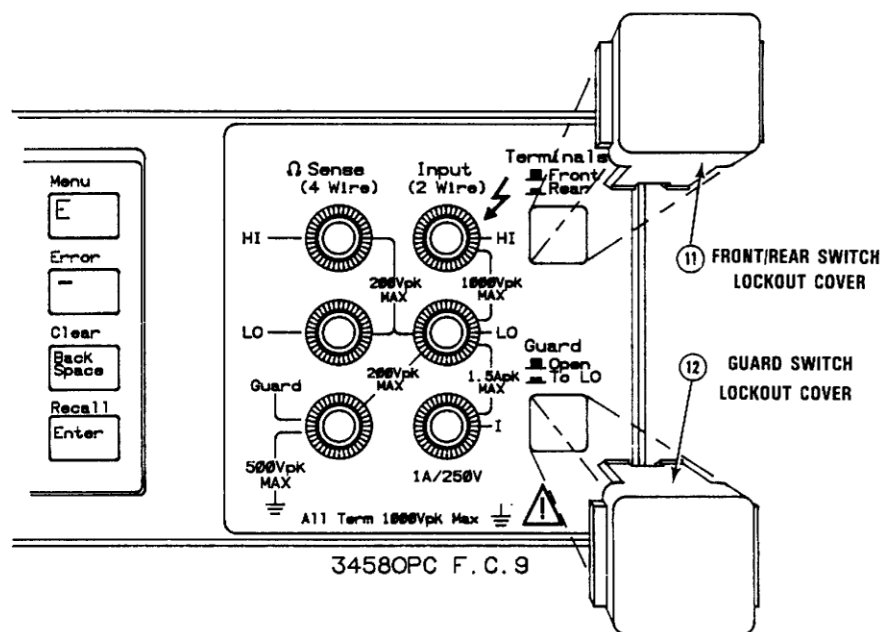
Figure 43. Switch covers installation
