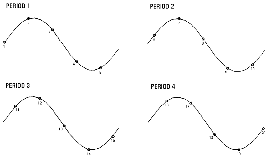
Figure 31. Sub-sampling example
