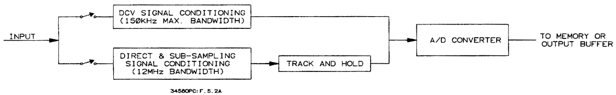
Figure 23. Digitizing signal paths
