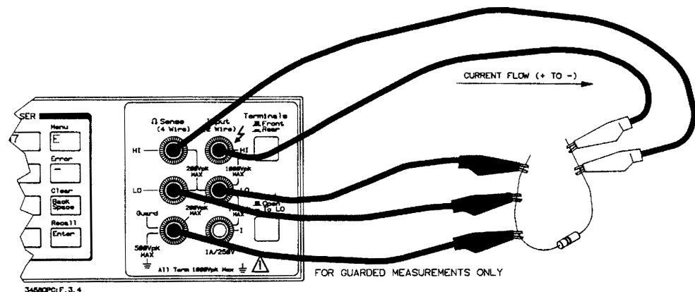
Figure 14. 4-Wire ohms measurement connections
