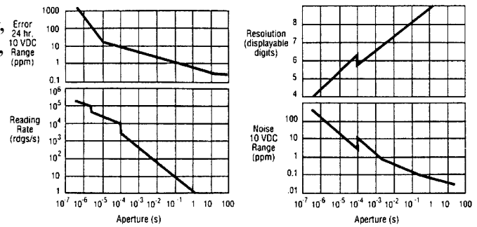
Figure 44. Shows the dependency of accuracy, reading rate, resolution, and noise on aperture or NPLC selected.
