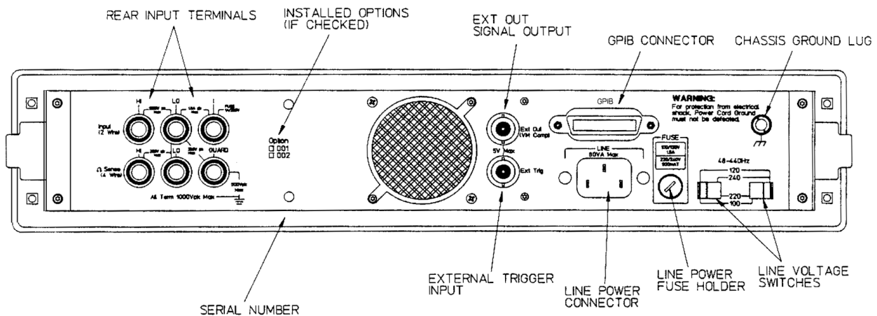
Figure 1. Rear panel
