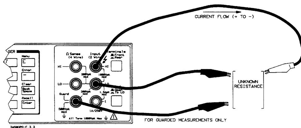
Figure 13. 2-Wire ohms measurement connections
