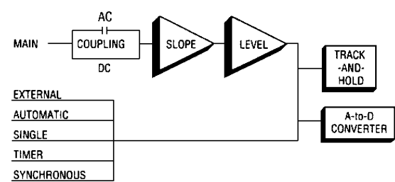
Figure 54. The trigger event choices shown provide the versatility needed to match a wide variety of applications.
