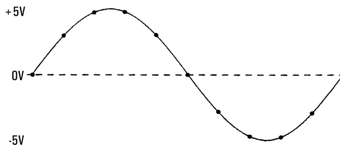
Figure 26. Level triggering at zero crossing, positive slope
