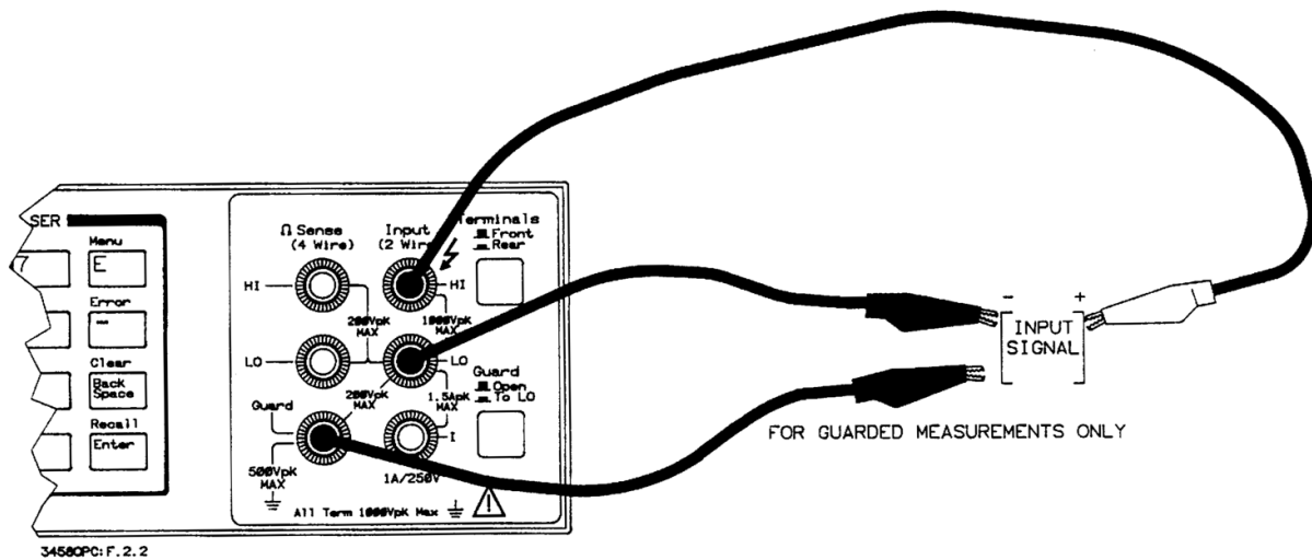
Figure 7. Standard 2-wire (plus guard) measurements
