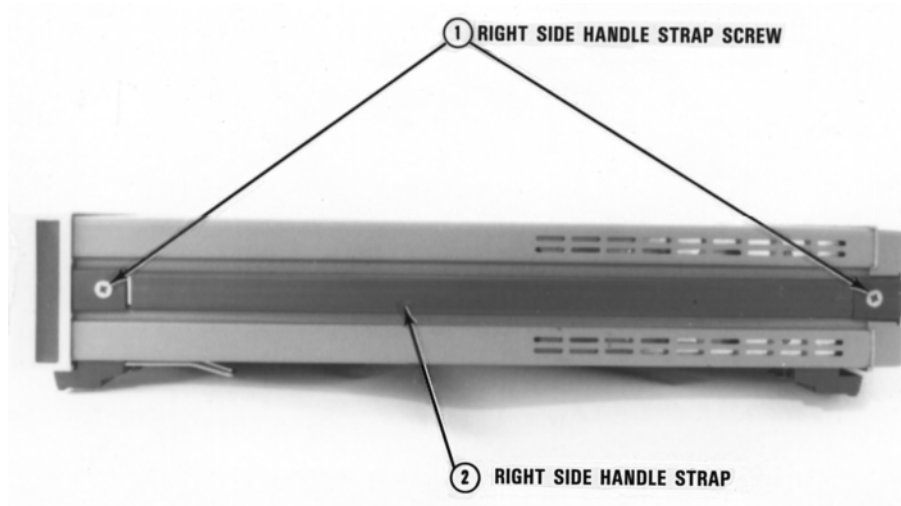
Figure 35. 3458 Right side
