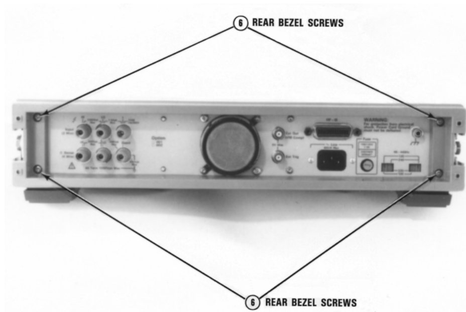
Figure 38. 3458 Rear view
