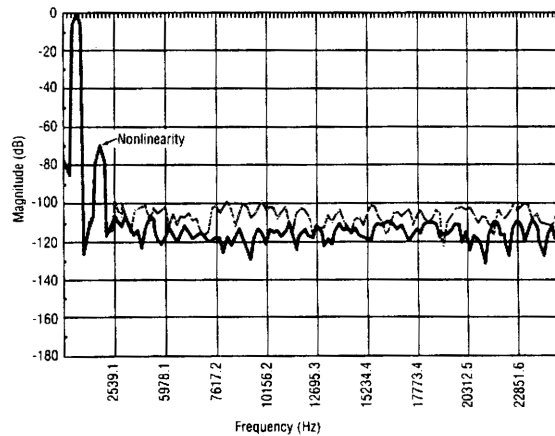
Figure 62. Analog-to-digital converters that exhibit non-linearity errors cause spurious responses that averaging will not remove. The 3458A is linear to 16 bits at 100,000 readings/s.
