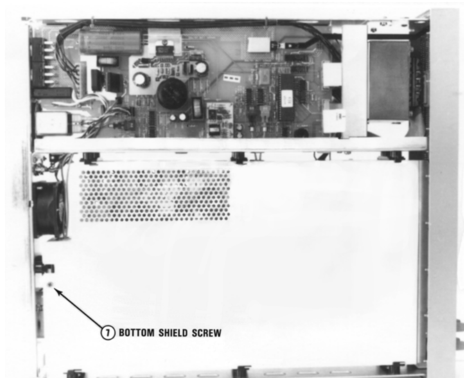
Figure 39. 3458 Inside bottom view
