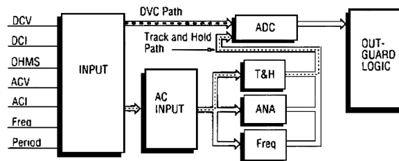
Figure 47. Signal path block diagram offers three techniques for ACV measurement.
