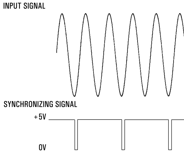
Figure 33. Typical synchronizing signal for EXT sync source
