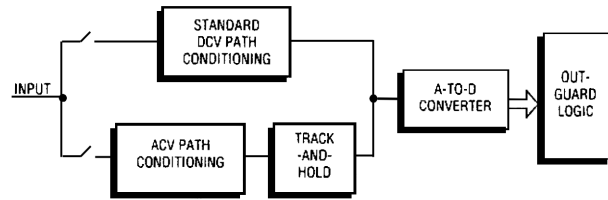
Figure 52. The 3458A Multimeter provides two different digitizing paths, the standard DCV path and a track-and-hold path.
