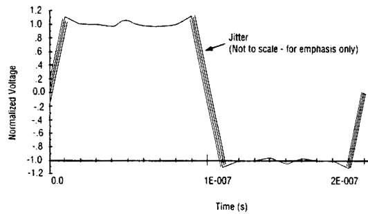
Figure 64. The effects of timebase jitter is shown here. For the 3458A Multimeter, the jitter is 50ps RMS. This jitter is repeatable so it can be characterized and corrected.
