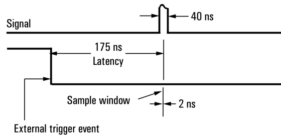
Figure 53. Capturing the pulse amplitude of narrow pulses requires the use of the 12 MHz track-and-hold path. Note, the minimum time between sample acquisition and trigger event is 175 nanoseconds.
