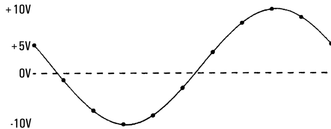
Figure 27. Level triggering, 50%, neg. slope, AC-coupled
