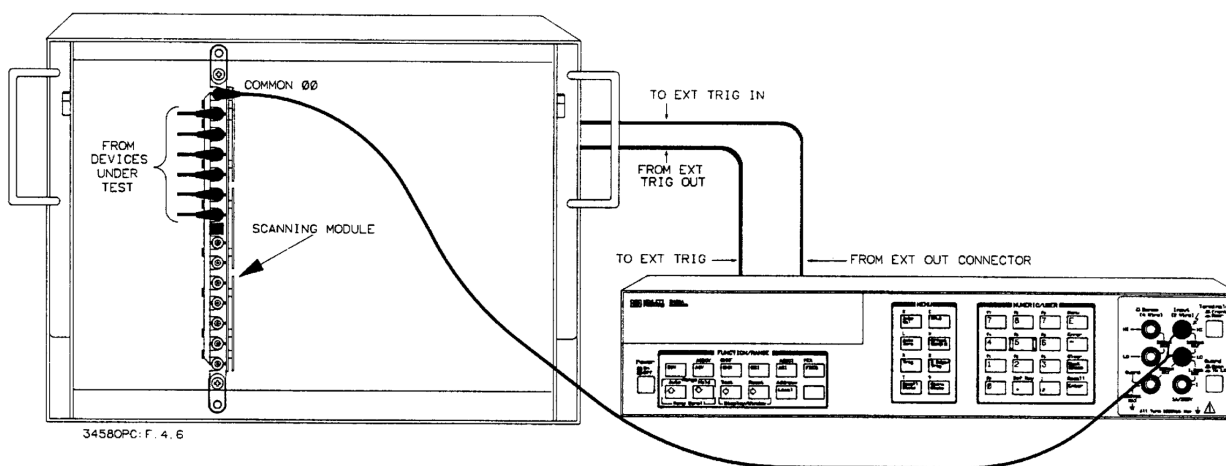
Figure 21. Using an external scanner
