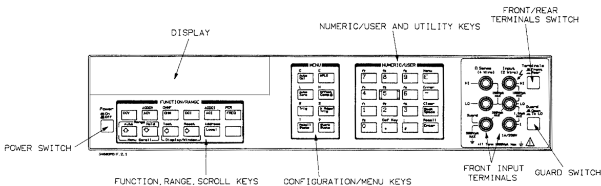
Figure 6. Front Panel
