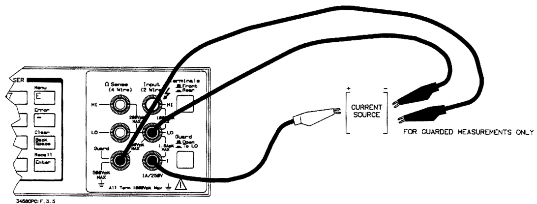
Figure 12. Current measurement connections
