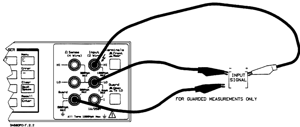
Figure 24. Digitizing measurement connections
