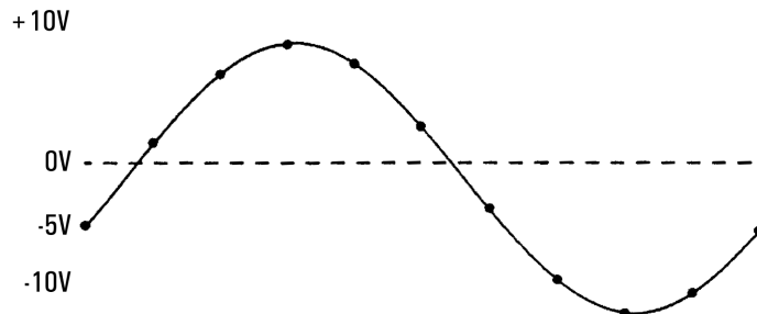
Figure 28. Level triggering, -50%, pos. slope, AC-coupled
