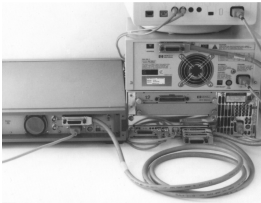
Figure 4. Typical GPIB Connections
