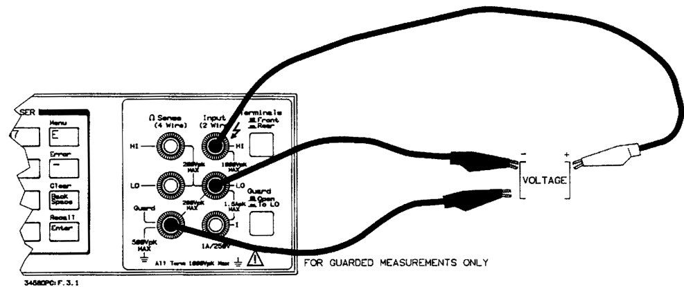
Figure 11. Voltage measurement connections
