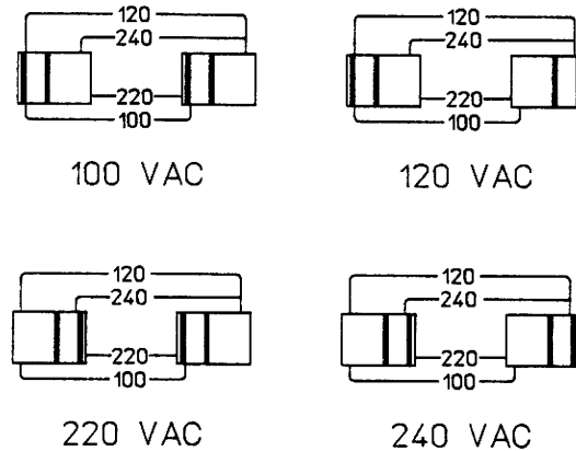
Figure 2. AC line voltage switch positions
