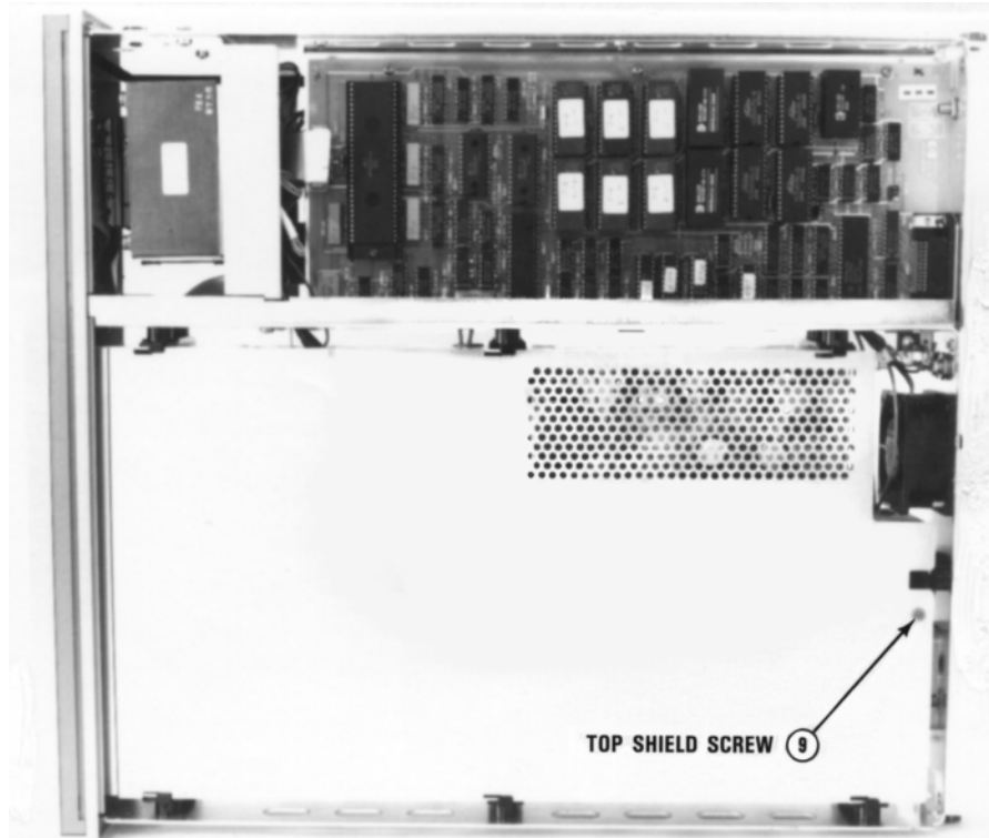
Figure 41. 3458 Inside top view
