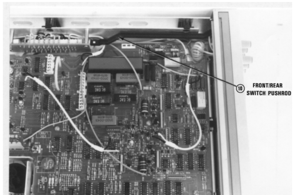
Figure 42. Front/rear terminal switch and pushrod location
