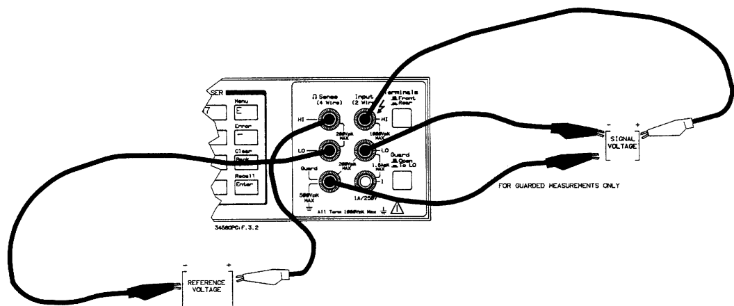
Figure 15. Ratio measurement connections
