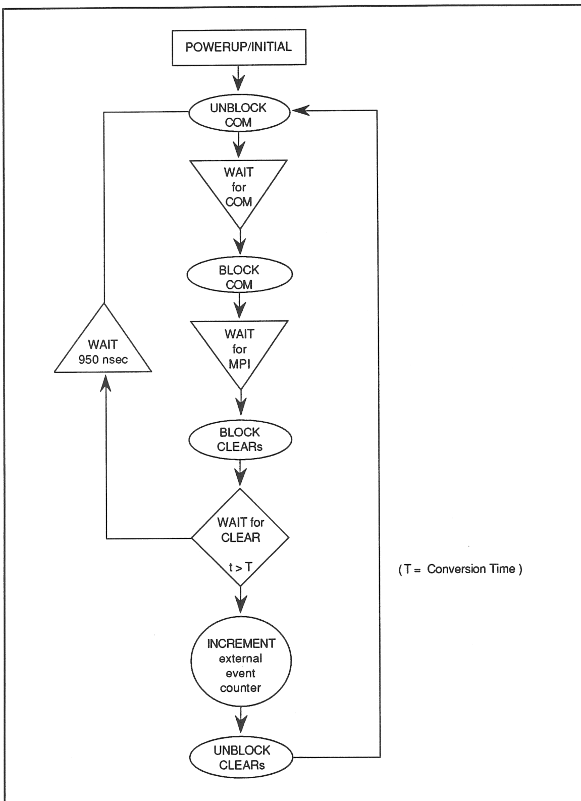
Figure 11 F Mode - Readout during next conversion with CLEAR blocked Hardware Logic
