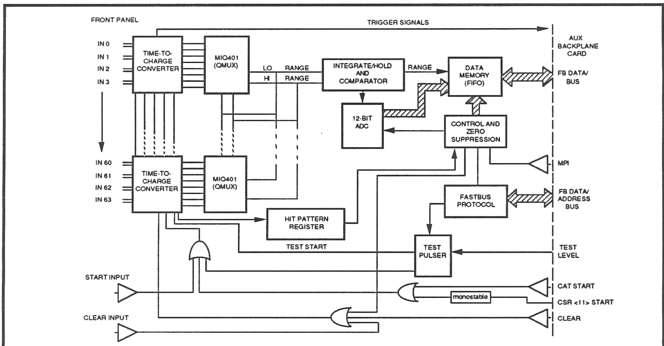
The Model 1875A Block Diagram
