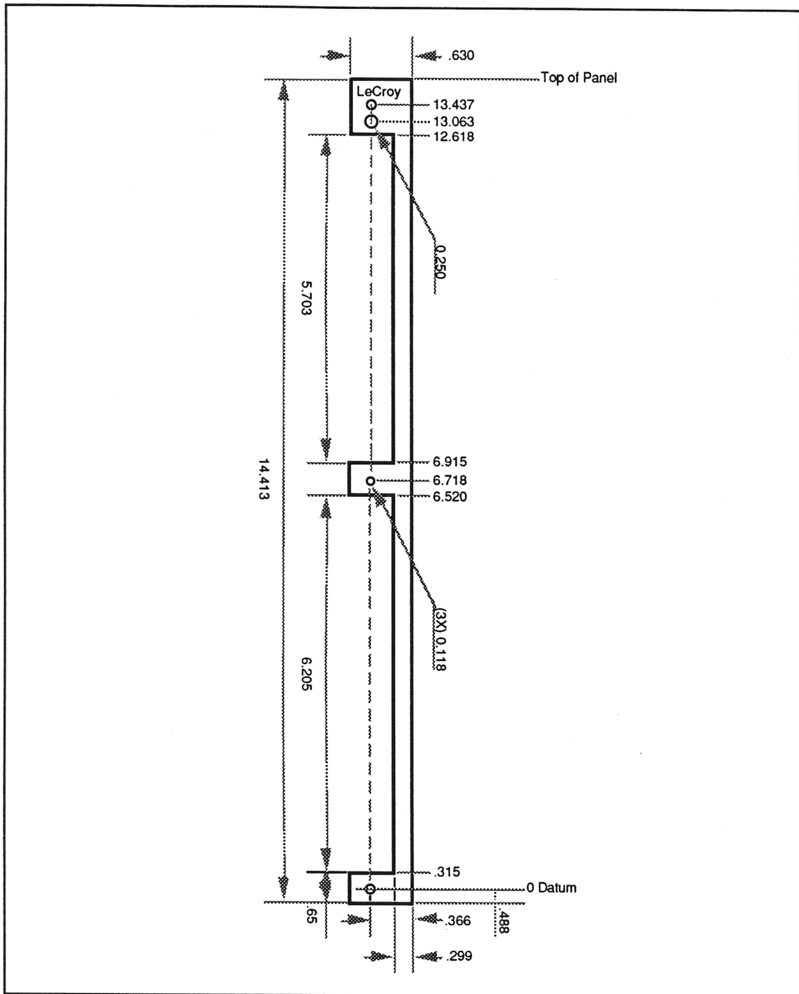
Figure 19 1872A/75A Front Panel
