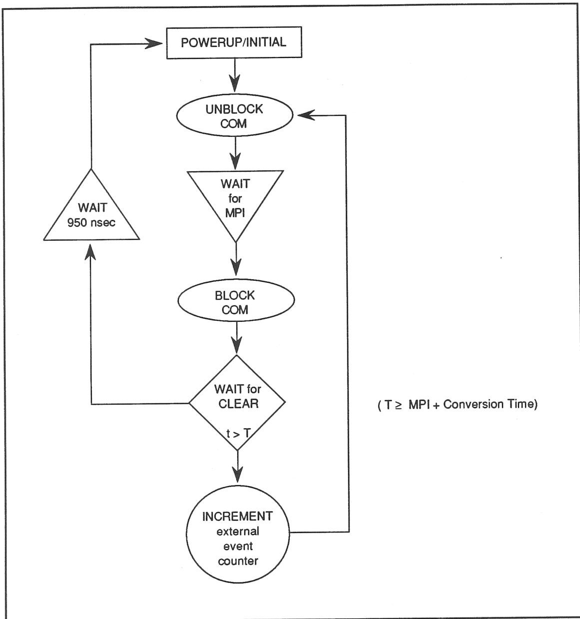
Figure 14 F Mode - Readout during next conversion Hardware Logic
