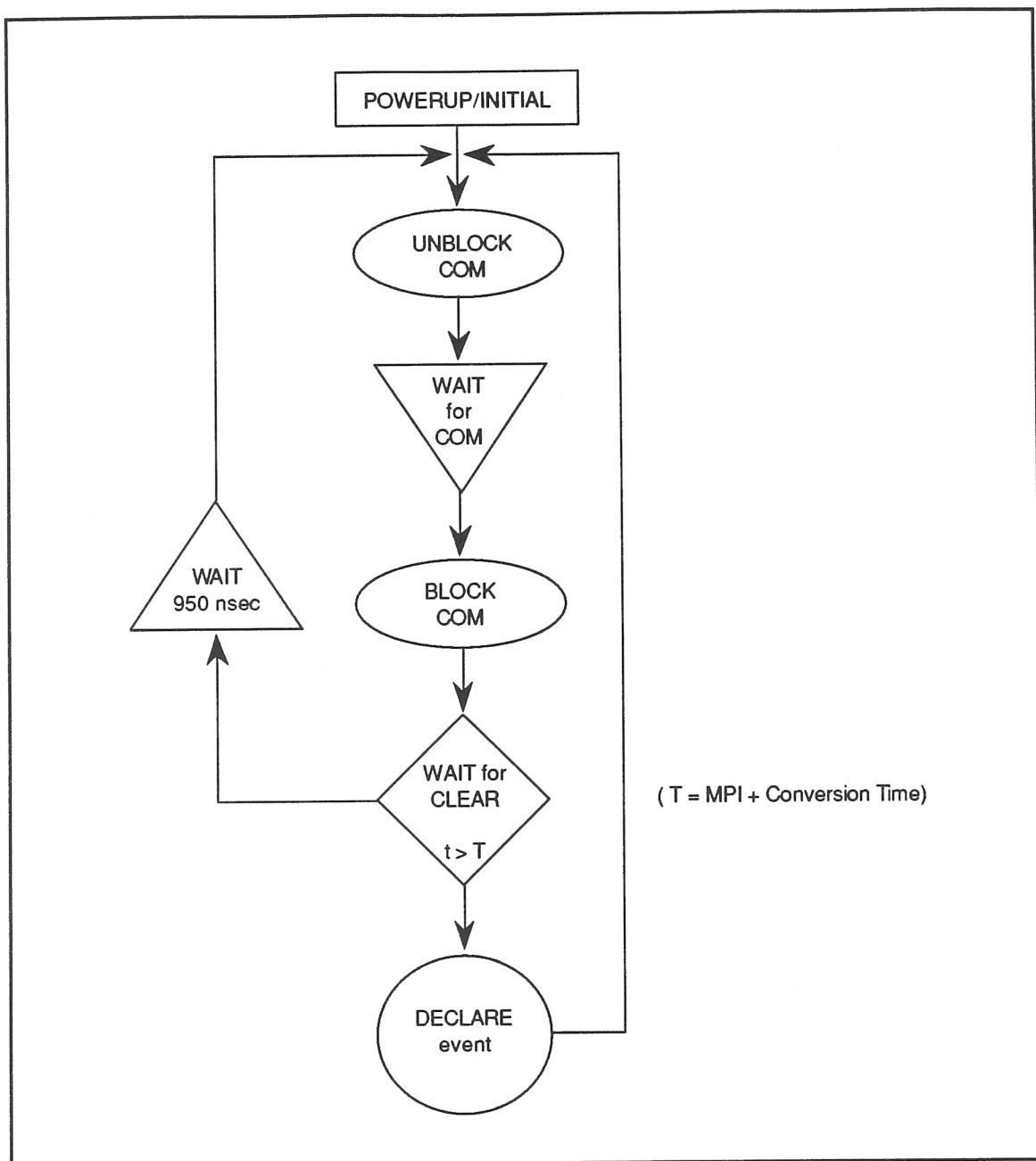
Figure 8 F Mode - Readout with next COM allowed Hardware Logic
