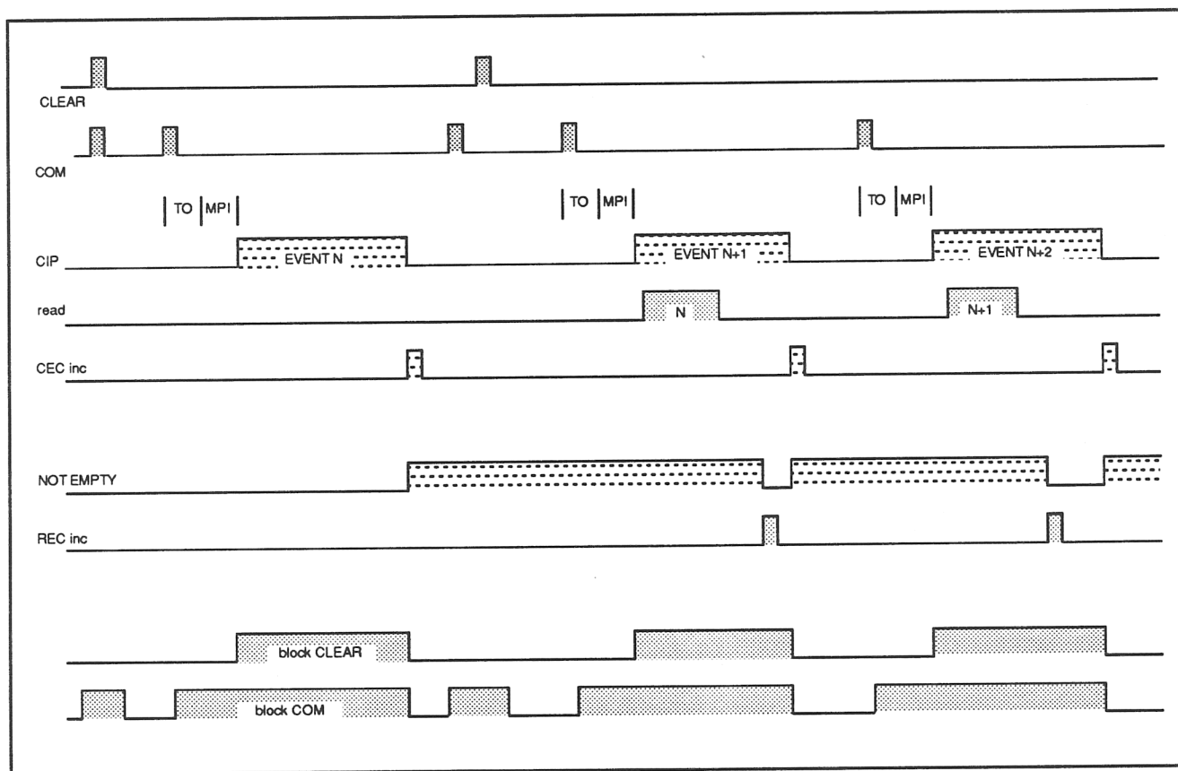
Figure 10 F Mode - Readout during next conversion with CLEAR blocked Timing Diagram
