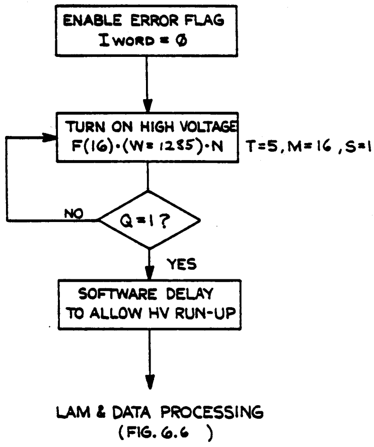
Figure 9: Sub-Routine 3; Turn On High Voltage
