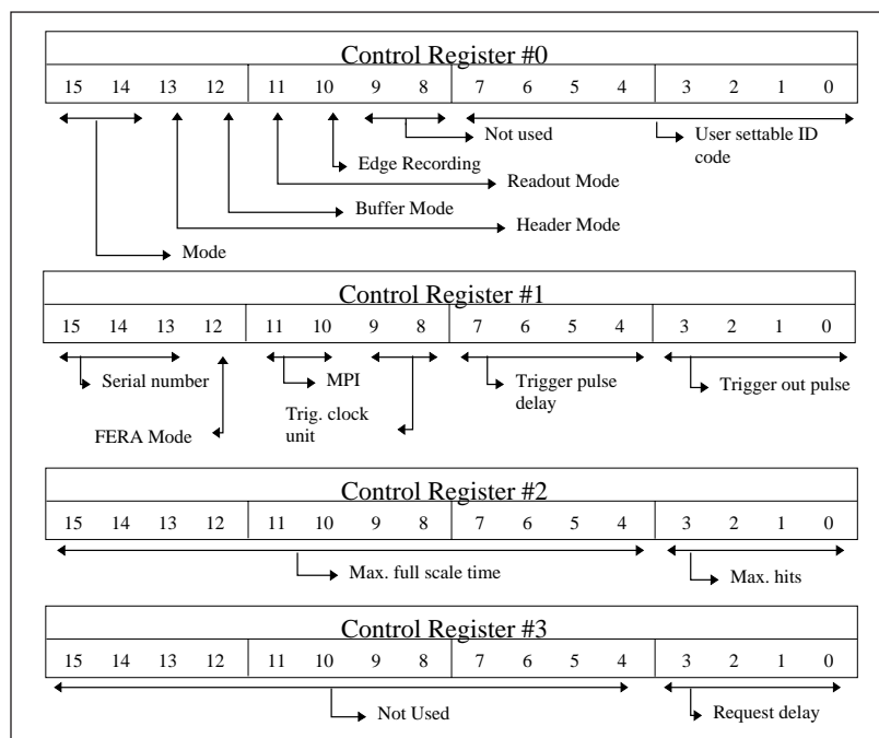
Mode 2 Control Registers
