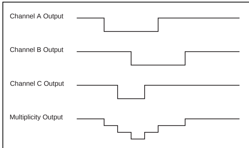
Figure 7: Multiplicity Waveforms
