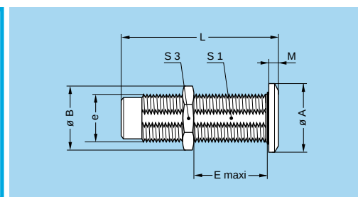
S●● Fixed coupler, nut fixing, key (G) or keys (A, B, J, K and L) at the flange end and key (G) or keys (A, B, J, K and L) at the other end, watertight or vacuumtight
