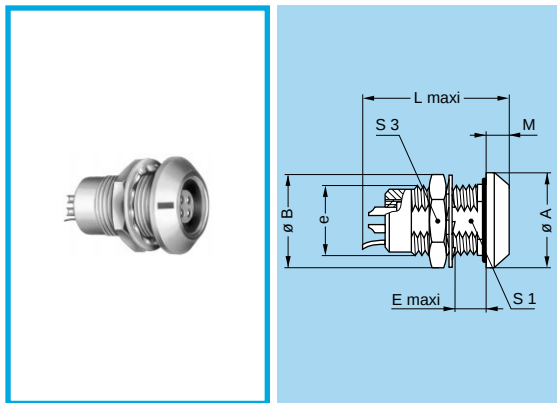
HNG Fixed socket, nut fixing, with earthing tag, key (G) or keys (A...M), watertight or vacuumtight
