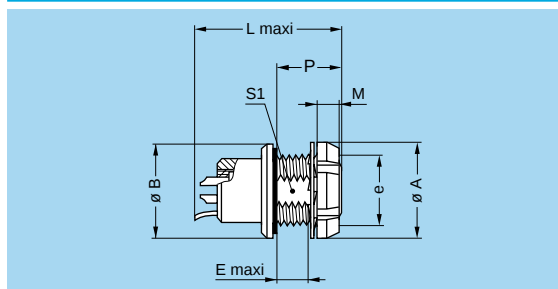
S●● Fixed coupler, nut fixing, key (G) or keys (A, B, J, K and L) at the flange end and key (G) or keys (A, B, J, K and L) at the other end, watertight or vacuumtight
