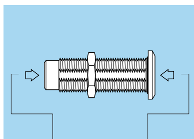
S●● Fixed coupler, nut fixing, key (G) or keys (A, B, J, K and L) at the flange end and key (G) or keys (A, B, J, K and L) at the other end, watertight or vacuumtight
