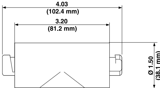
Multi-Way Connector – Male To Male
