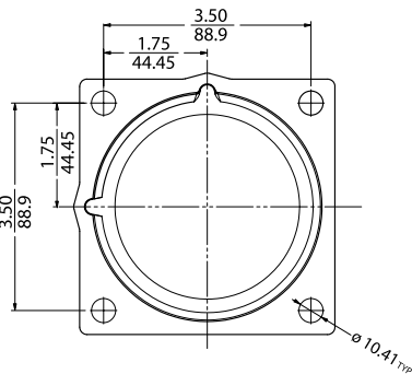
Panel Receptacle Flange
