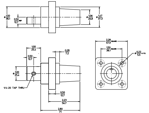
16R20 Female Panel Receptacle Buss Bar Version
