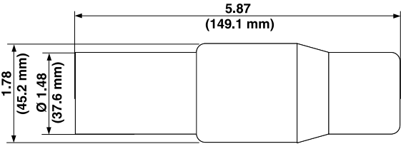
Male Vulcanized Plug – Crimped
