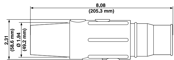
Female Plug - Double Set Screw Detachable
