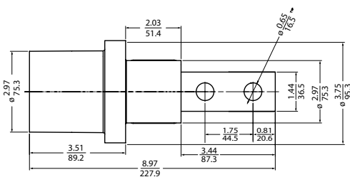
Female 2-Hole Bus Bar
