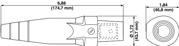
Female Detachable Plug – Single Set Screw
