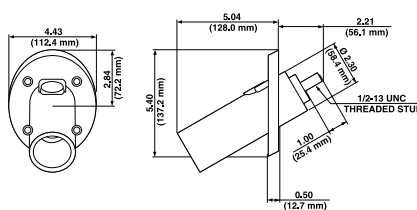
Male Panel Receptacle Threaded Stud – 30°
