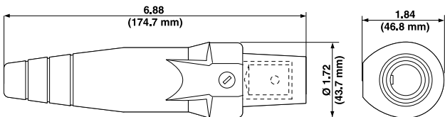
Female Detachable Plug – Crimped
