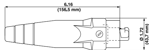
Male Detachable Plug – Single Set Screw
