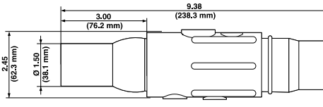
Ball Nose In-line Latching Female Connectors - Crimped
