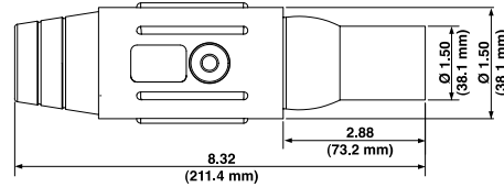
Ball Nose In-line Latching Female Connectors S-Series
