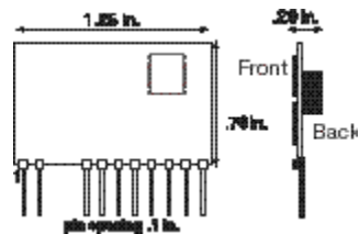
Figure 10: Physical package
