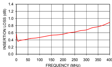
ADT1-1WT-1 INSERTION LOSS
