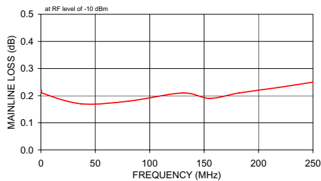
ZFDC-20-3+ MAINLINE LOSS
