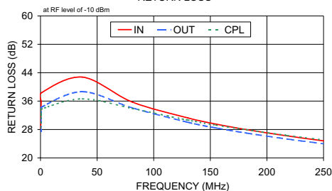
ZFDC-20-3+ RETURN LOSS
