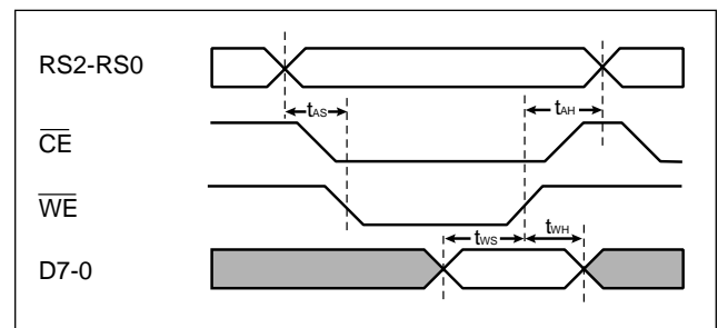
Figure 7. CPU Write
