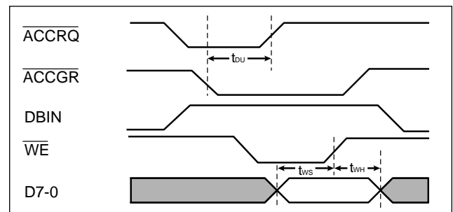
Figure 8. DMA Write
