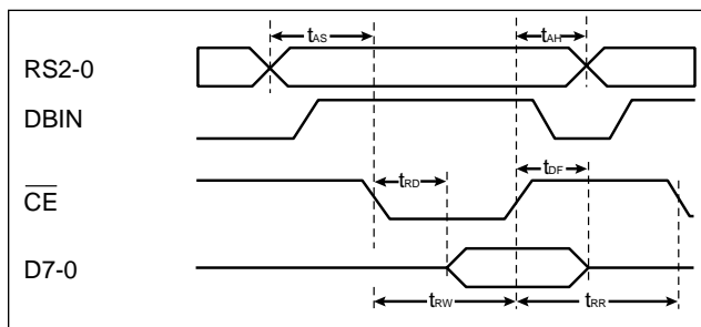
Figure 5. CPU Read
