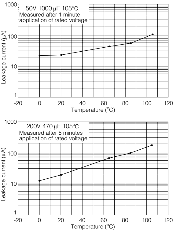
Fig. 1 - 12 Leakage current vs. Temperature Characteristic
