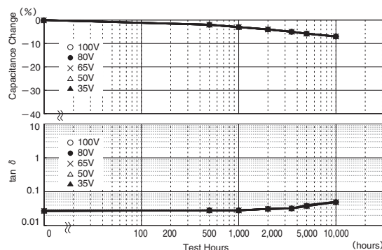
Fig-20 Endurance (measured by each apply voltage, result curves are overlapped) Note: Due to the very small effect of the applying voltages, the plots cannot be distinguished from one another.
