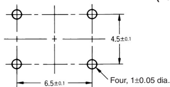
PCB Mounting (Top View) (Single-sided PCB, t=1.6)
