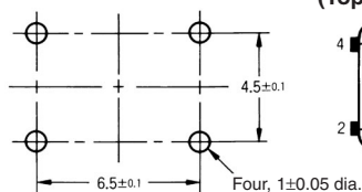
PCB Mounting (Top View) (Single-sided PCB, t=1.6)
