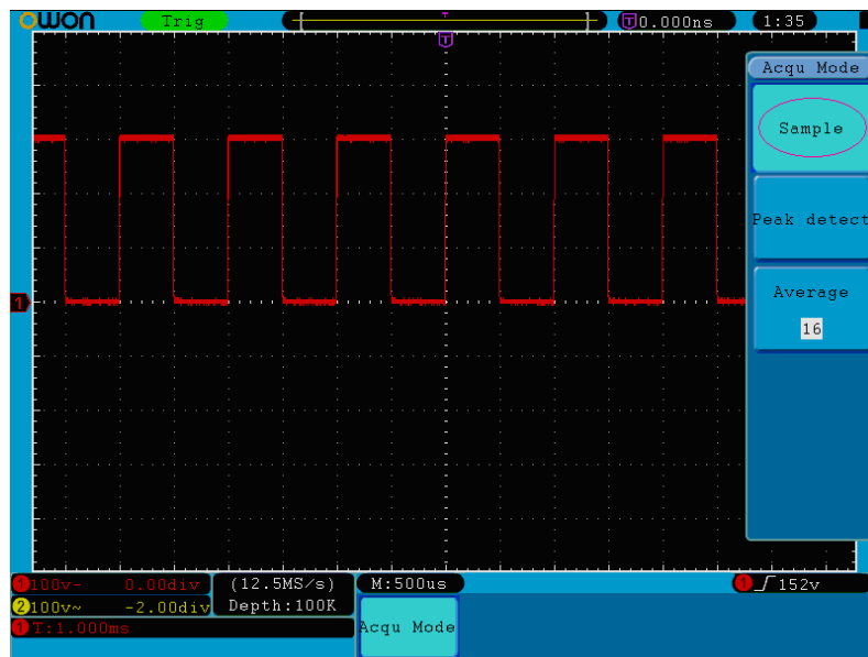
Figure 5-27 Normal ACQU Mode display, in which no burr can be detected.
