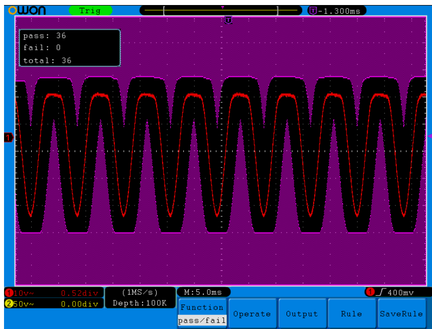
Figure 5-55 Pass/Fail test
