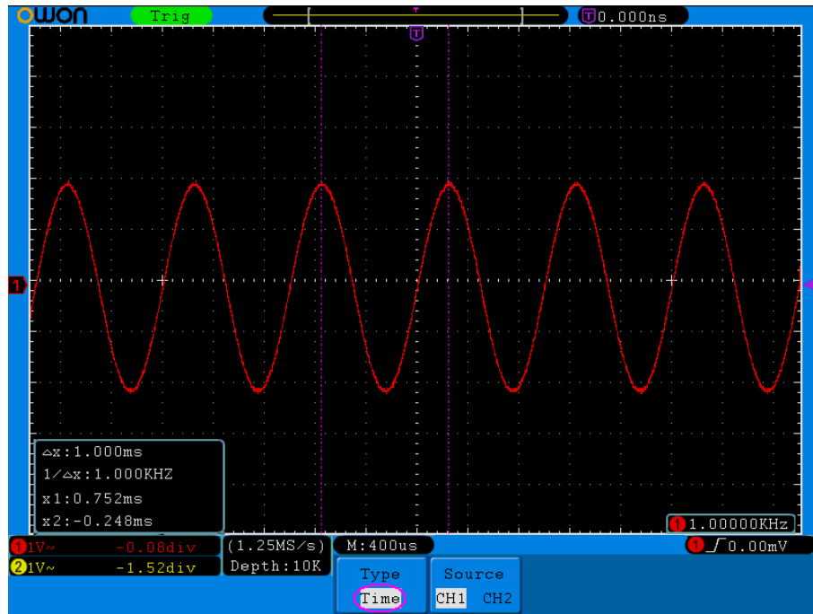
Figure 5-64 Waveform of Cursor Measurement
