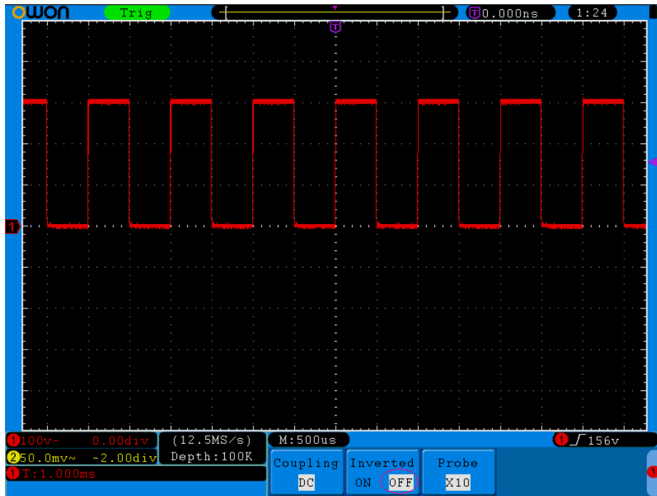
Figure 5-4 Original Waveform
