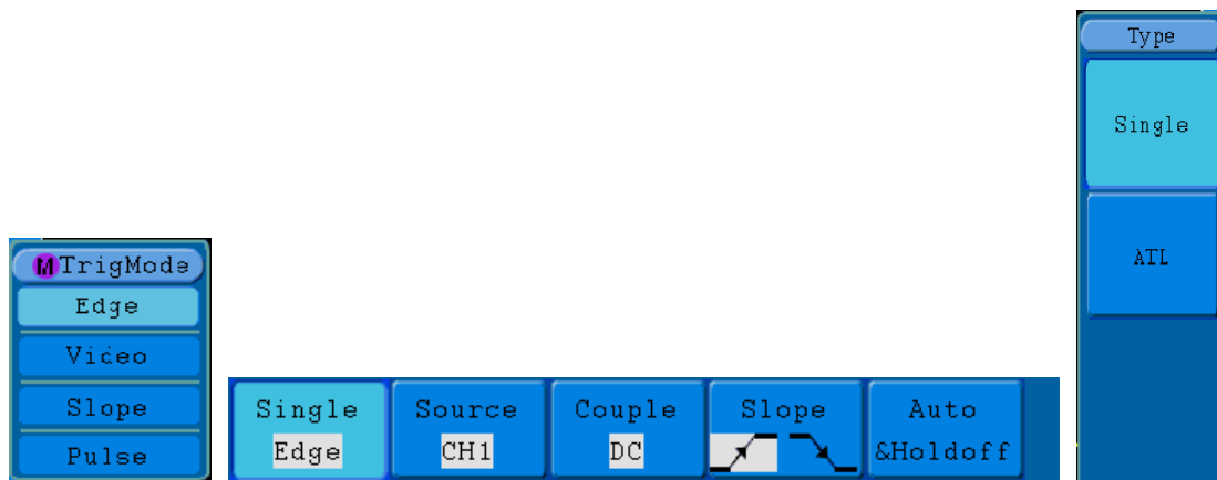
Figure 5-17 Edge trigger menu (SDS5032E(V)) does not support alternate trigger)
