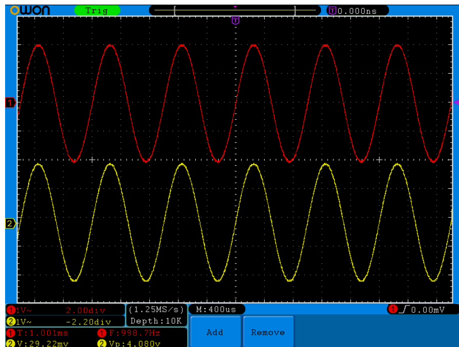
Figure 5-59 automatic measurement
