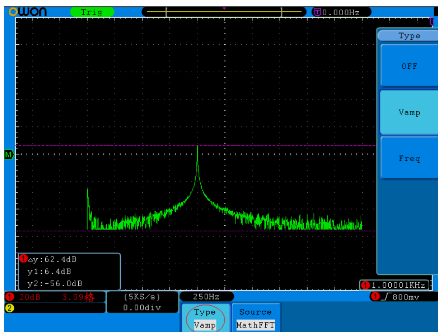
Figure 5-66 wave of Vamp cursor measurement
