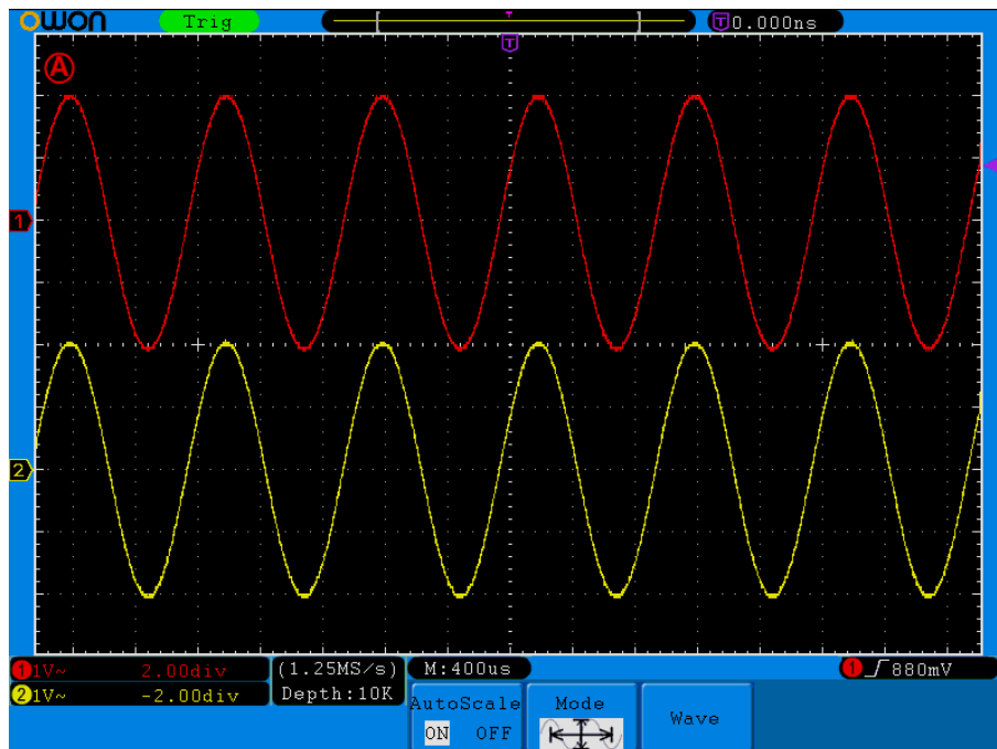
Figure 5-69 Autoscale Horizontal-Vertical multi-period waveforms
