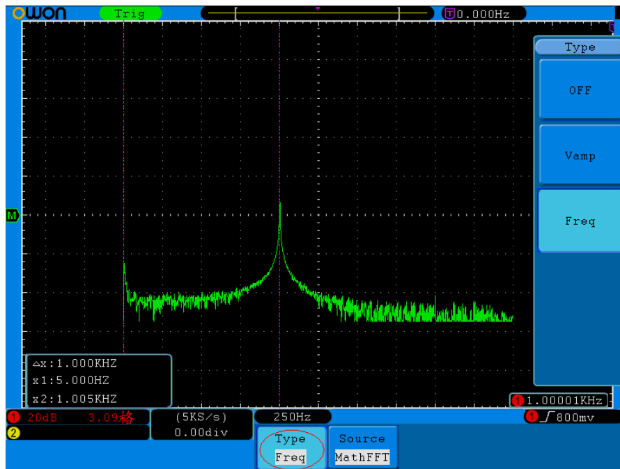
Figure 5-67 wave of Freq cursor measurement
