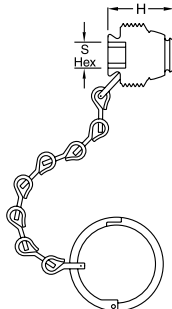
CGA Plug 510, 580 & 590
