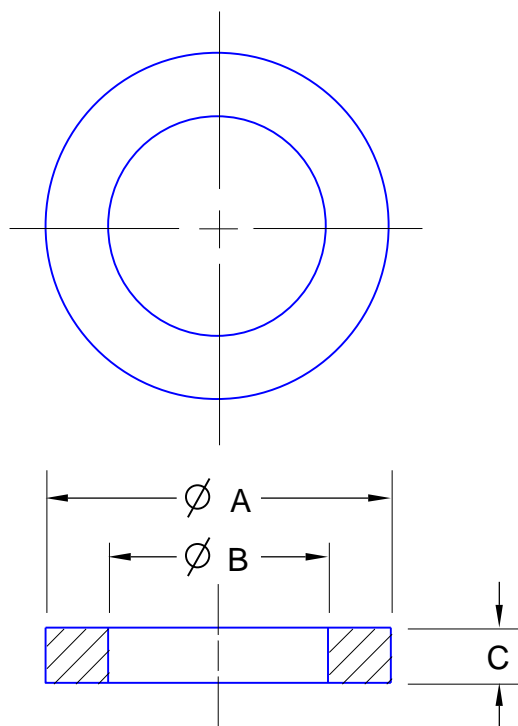
FIGURE 4. Gasket.
