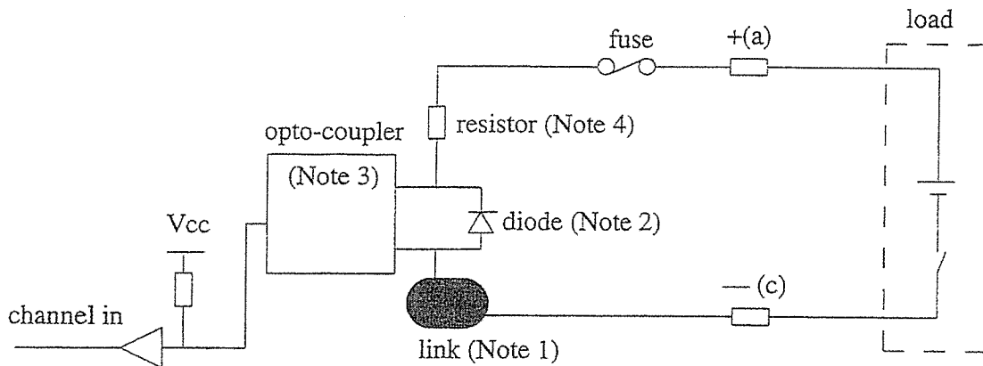
Figure 7. Input Circuit
