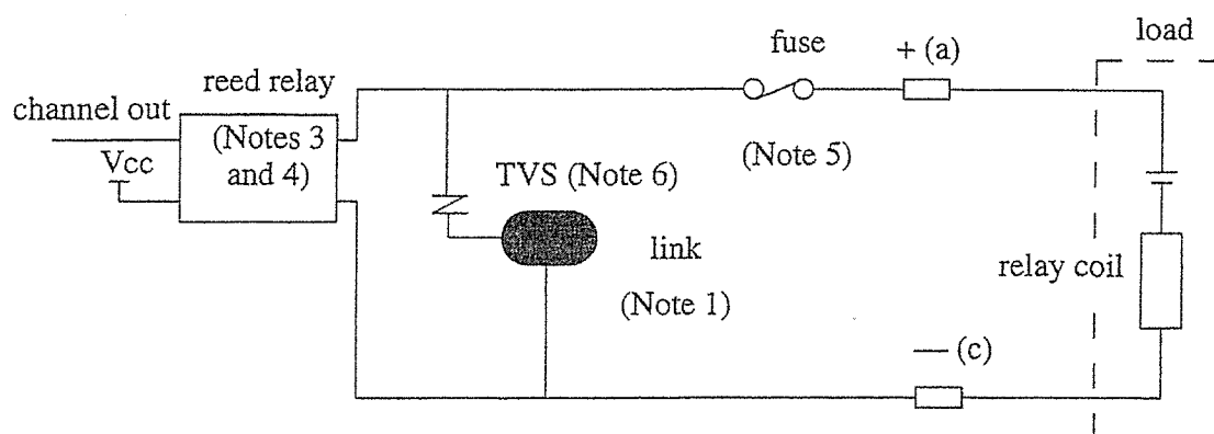
Figure 9. Output Circuit
