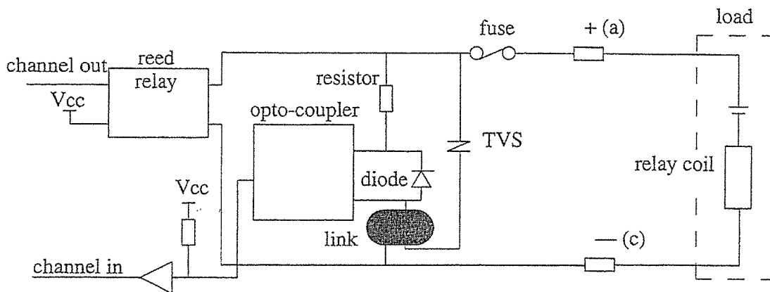
Figure 6. Input/Output Circuit
