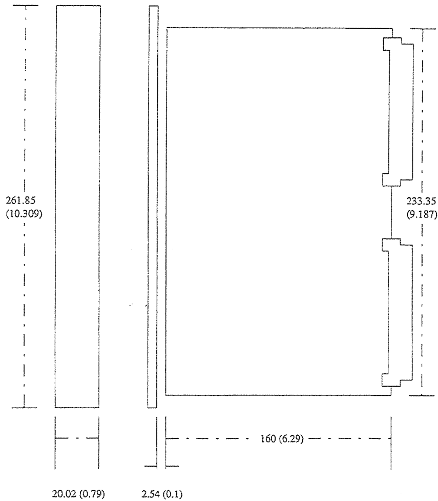
Figure 2. VME Dimensions
