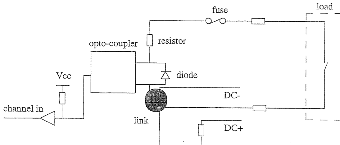
Figure 8. Self Powered Input on Channels 17 to 32
