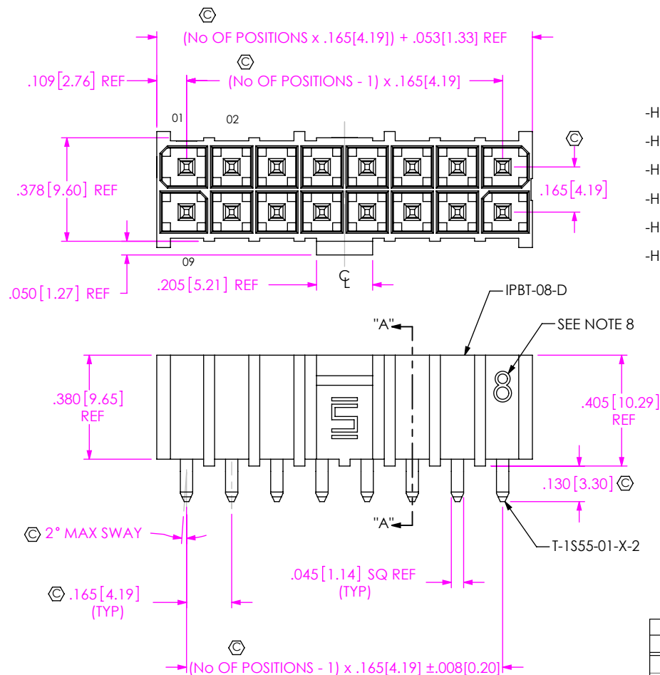
FIG. 1 (IPBT-108-H1-XX-D SHOWN)
