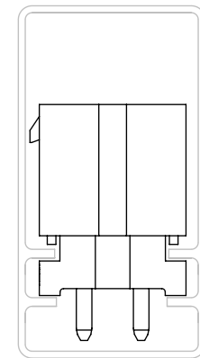
IPBT-1XX-H4-XX-D-XX SHOWN TUBE: PT-IPBT001-H4-H6 PLUG: TP-28
