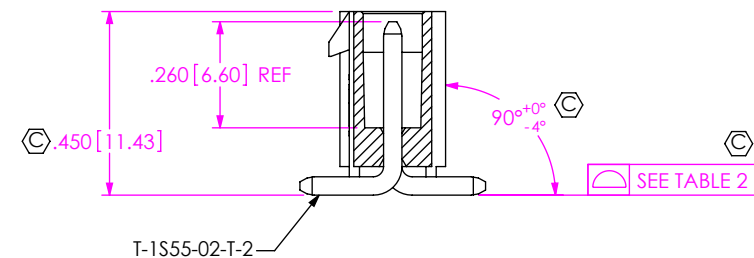
FIG 3 STYLE -H2: SURFACE MOUNT (IPBT-108-H2-XX-S SHOWN) (DIFFERENT AS SHOWN, OTHERWISE SAME AS FIG 1)
