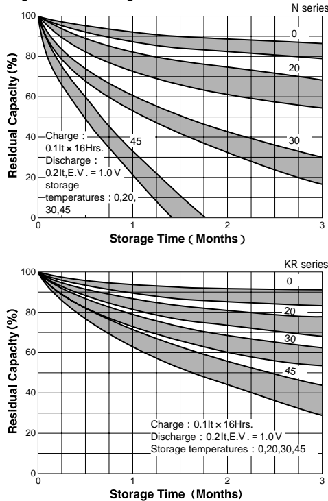
Fig.4-1: Storage Characteristics
