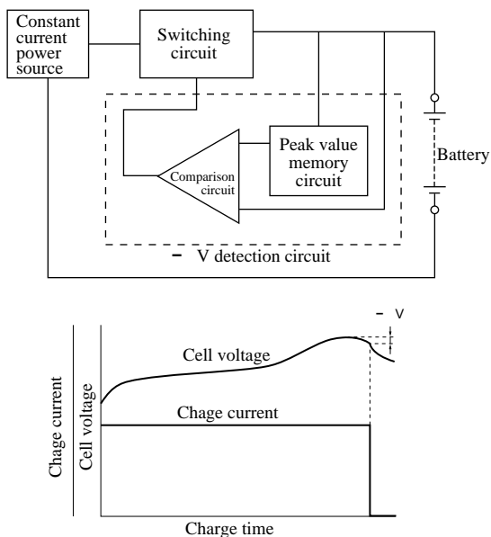
Fig.8-11: - \Delta V Detection Control System
