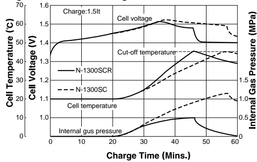
Fig.6-5: Fast-Charge Characteristics
