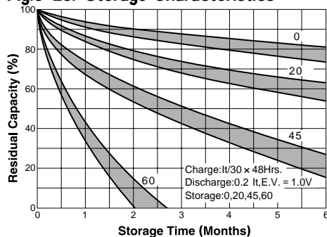
Fig.6-26: Storage Characteristics
