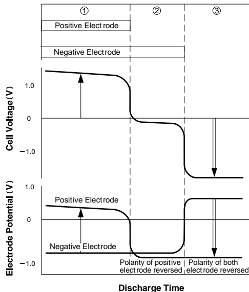
Fig.3-10: Polarity Reversal
