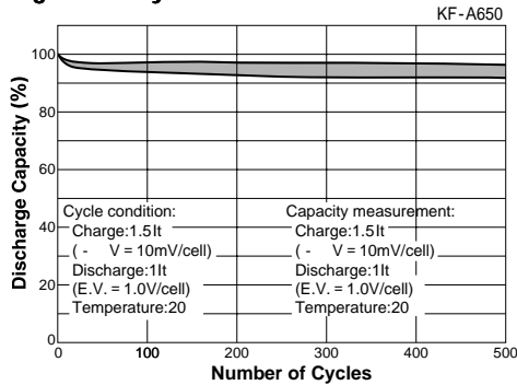
Fig.7-6: Cycle Characteristics
