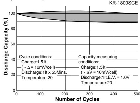
Fig.6-4: Cycle Characteristics
