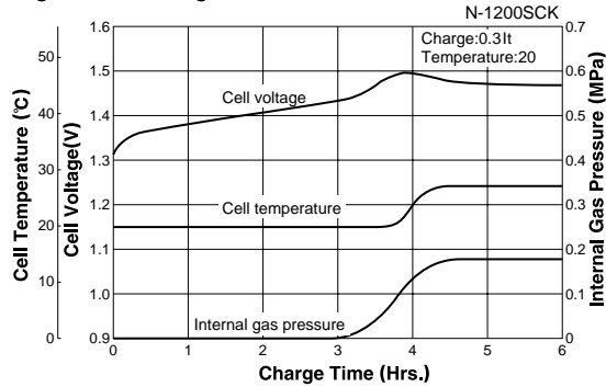
Fig.6-18: Charge Characteristics
