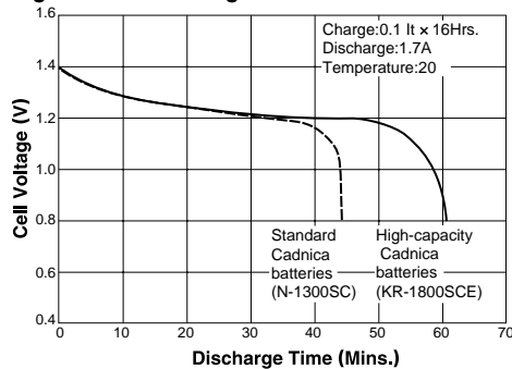
Fig.6-2: Discharge Characteristics
