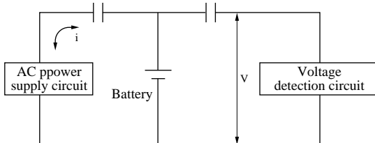
Fig.3-5: Measuring Internal Resistance by Alternating-Current Method
