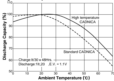
Fig.6-13: Temperature Characteristics
