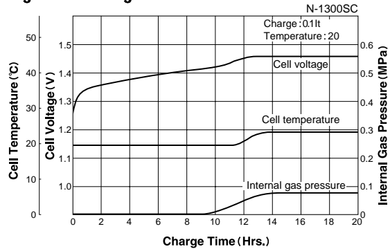
Fig.2-1: Charge Characteristics
