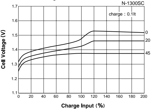
Fig.2-11: Ambient Temperature and Cell Voltage
