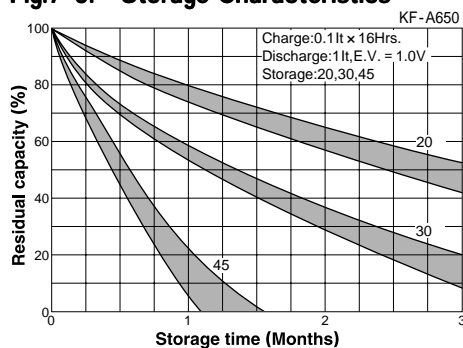
Fig.7-5: Storage Characteristics
