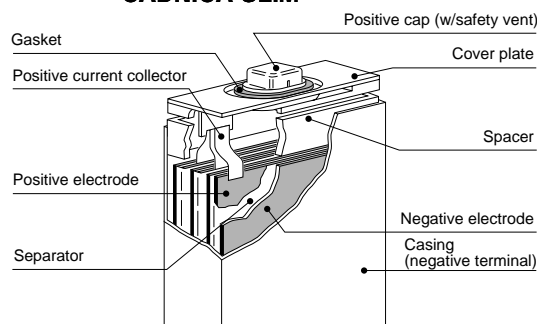
Fig.7-1: Structural Design of CADNICA SLIM
