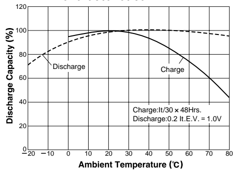
Fig.6-27: Temperature Characteristics
