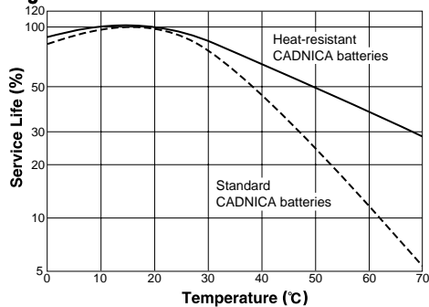
Fig.6-21: Service Life
