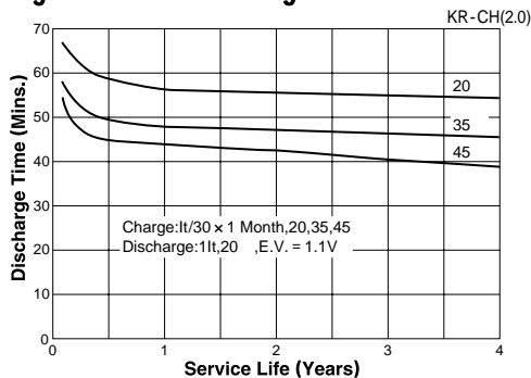
Fig.6-17: Trickle Charge Service Life
