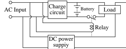
Fig.8-4: Trickle Charging Circuit
