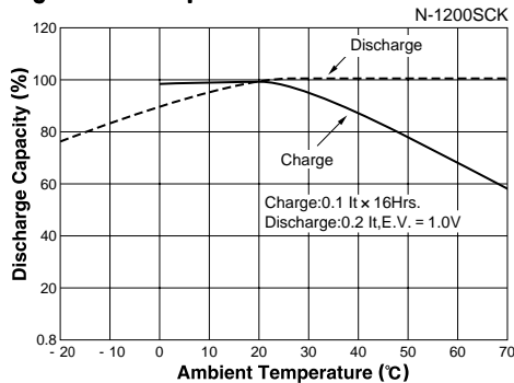
Fig.6-20: Temperature Characteristics
