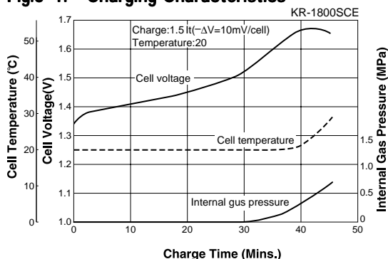
Fig.6-1: Charging Characteristics
