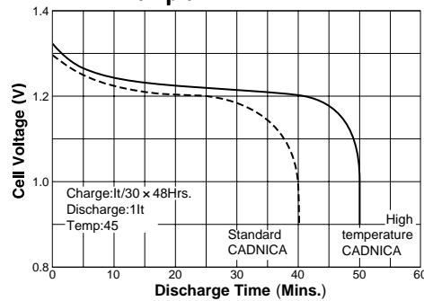
Fig.6-15: High Temperature Trickle-Charge Characteristics Example A
