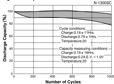
Fig.5-2: Cycle Characteristics
