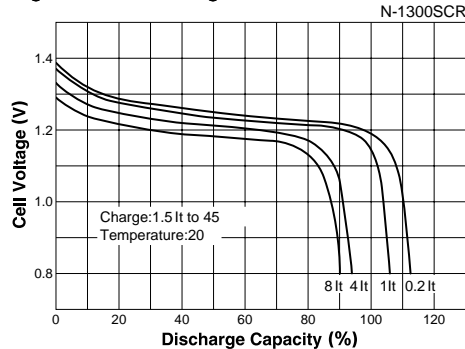
Fig.6-8: Discharge Characteristics
