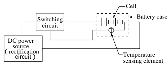
Fig.8-12: Cell Temperature Detection System
