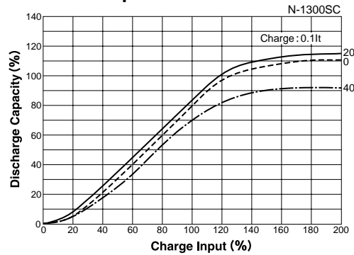
Fig.2-4: Charge Efficiency vs Ambient Temperature
