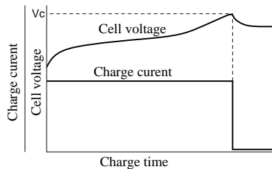
Fig.8-10: Cell Voltage Detection
