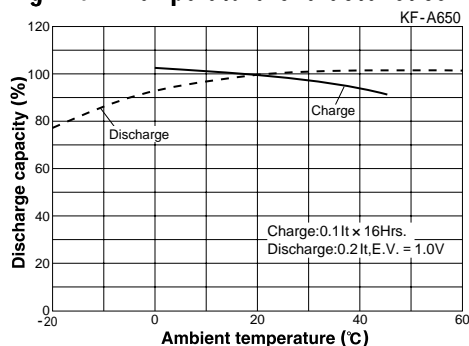
Fig.7-4: Temperature Characteristics
