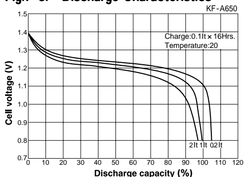
Fig.7-3: Discharge Characteristics
