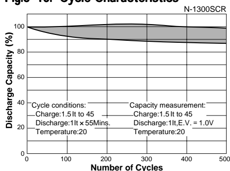
Fig.6-10: Cycle Characteristics
