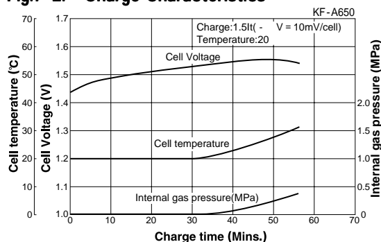
Fig.7-2: Charge Characteristics
