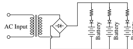
Fig.8-14: Parallel Charging Circuit
