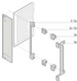
Diagram shows all fixing options for PCB bracket; Item 5c shows the product selected
