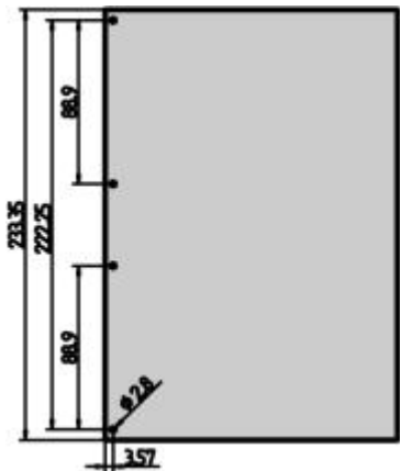
Drill hole dimensions on PCB, 3 U
