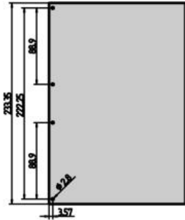
Drill hole dimensions on PCB, 6 U
