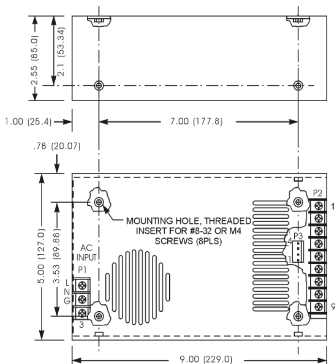
Dimensions (inches/mm) for 200 Watt, GL Series
