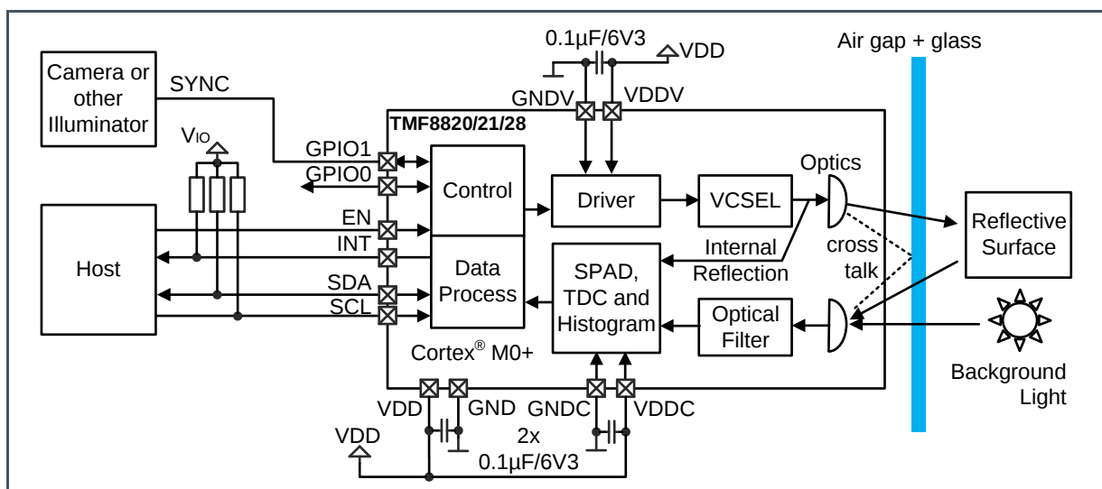
Figure 146: TMF8820/21/28 Application Schematic
