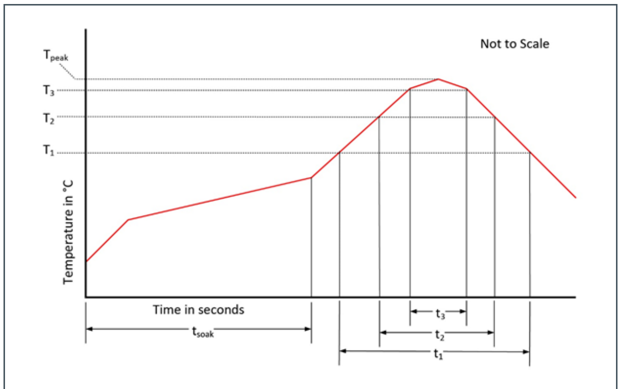
Figure 152: Solder Reflow Profile Graph
