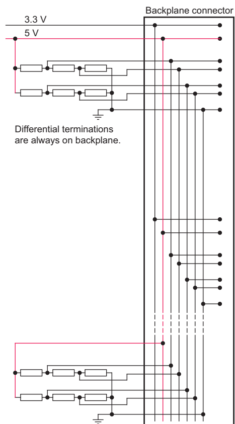
Fig 10. Hot swap application
