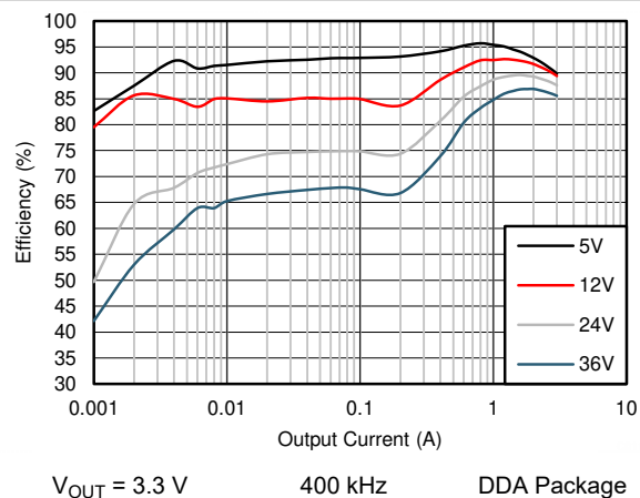
Figure 9-8. Efficiency
