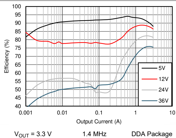
Figure 9-10. Efficiency
