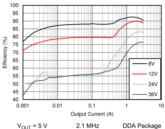
Figure 9-11. Efficiency
