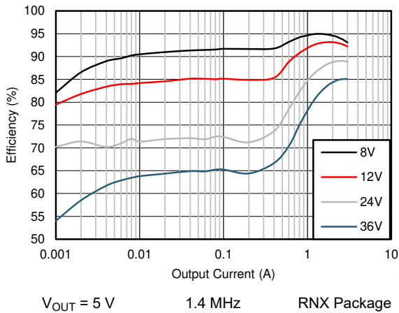
Figure 9-15. Efficiency
