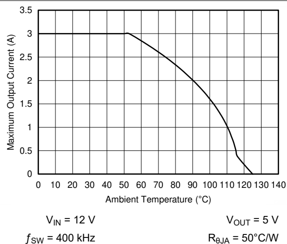
Figure 9-6. Maximum Output Current versus Ambient Temperature
