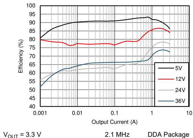
Figure 9-12. Efficiency
