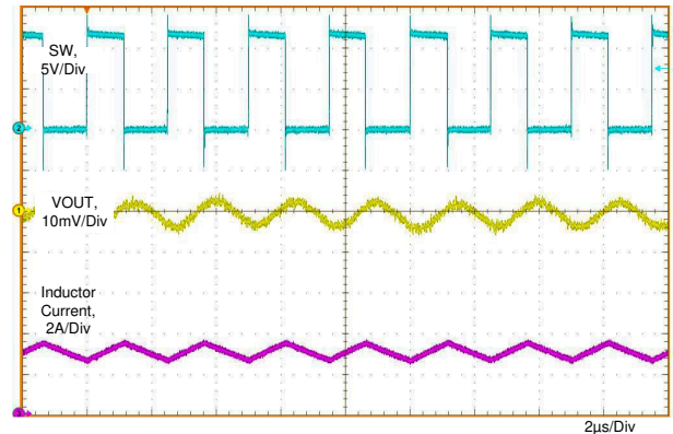
Figure 8-8. Typical PWM Switching Waveforms V_{IN} = 12\text{ V} , V_{OUT} = 5\text{ V} , I_{OUT} = 3\text{ A} , f_s = 400\text{ kHz}
