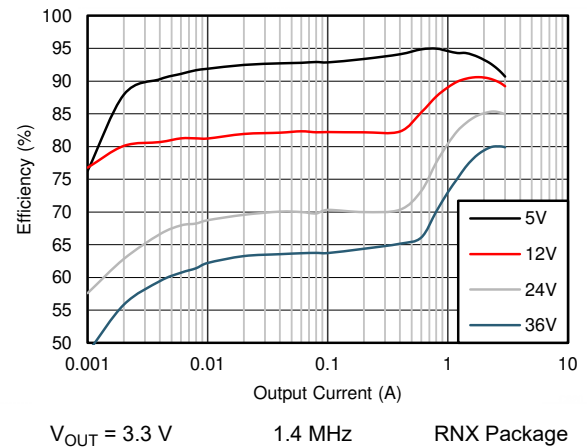
Figure 9-16. Efficiency
