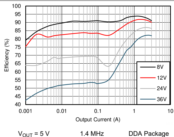
Figure 9-9. Efficiency
