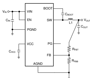
Simplified Schematic
