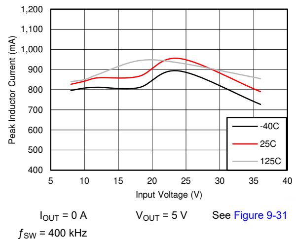
Figure 7-6. I_{PEAK-MIN}
