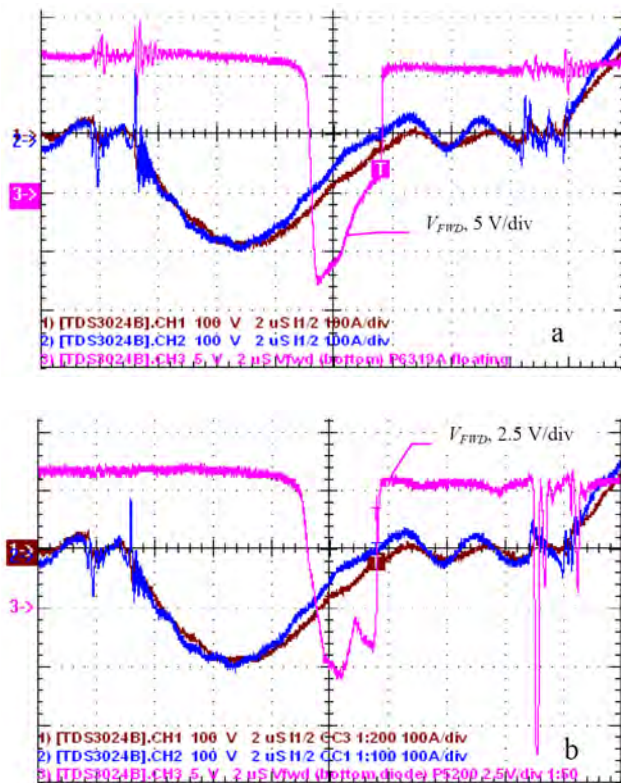
Fig. 11. Trace 3 - Forward drop of FWD IXYS DSEI 2x 61, two modules in parallel. a – high-bandwidth P6139A probe, b – differential probe. Both measurements taken with floating scope.
