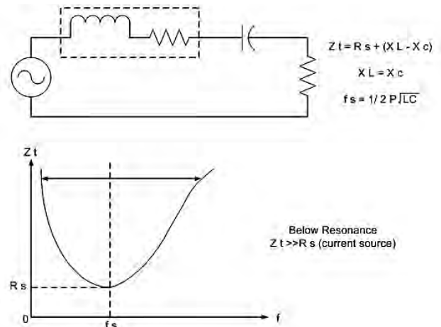
Fig. 6 Series Resonance
