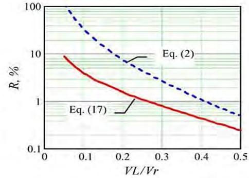
Fig. 9. Repeatability as a function of charge voltage, C_s = 200 \text{ nF} , C1 = C2 = 2 \mu\text{F} , worst case.
