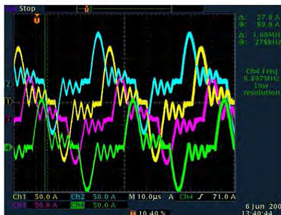
Fig. 7. Same as in Fig. 6 at 100 kV and 50 kW. Low-line voltage: 400 VAC-14% (345 VAC).
