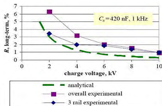
Fig. 17. Long-term repeatability as a function of charge voltage—summary of analytical calculations and experimental results.
