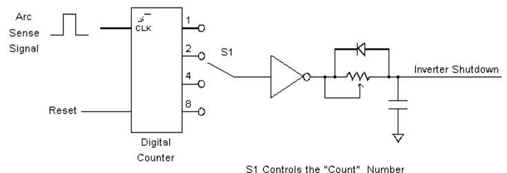
Fig. 5 Arc Count
