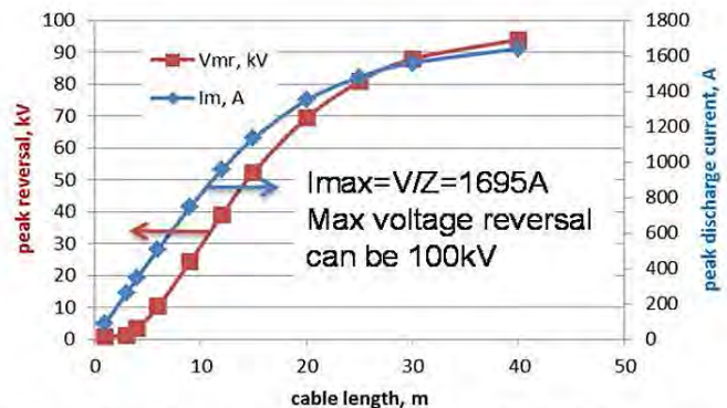
Figure 2. Dependence of peak reversal voltage ( V(T1:A+) ) and peak discharge current ( IB(T1) , respectively, per notation of Figure 1) on cable length (referenced to charge voltage of 100 kV). In these simulations, TTRAN=1 \mu s (actual transition from 90% to 10% is 200ns).
