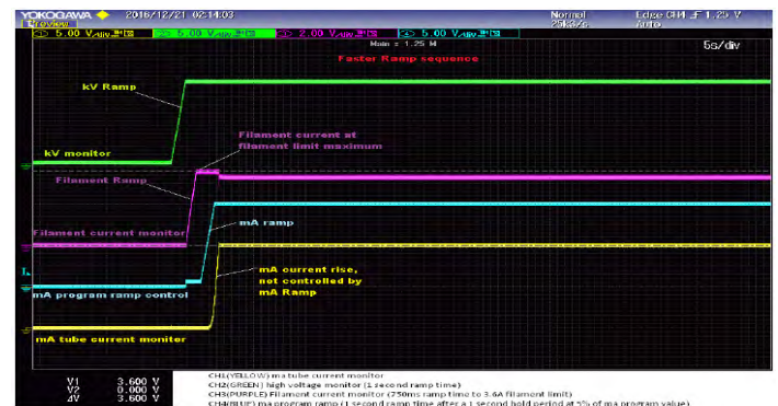
Figure 4: Filament and output currents during fast ramp.
