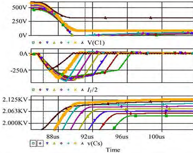
Fig. 7. Programmed charge voltage 2 kV. V_t = 460 \text{ V}, 480 \text{ V}, \dots, 600 \text{ V} . C_s = 200 \text{ nF} . Primary current I_1 is halved. Curves corresponding to largest overshoot are in thicker lines.
