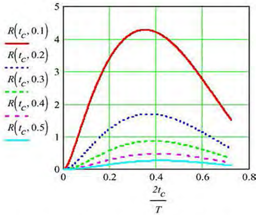
Fig. 23. Repeatability R\% versus chopping point t_c , with normalized load voltage v_l as a parameter. T = 2\pi/\omega .
