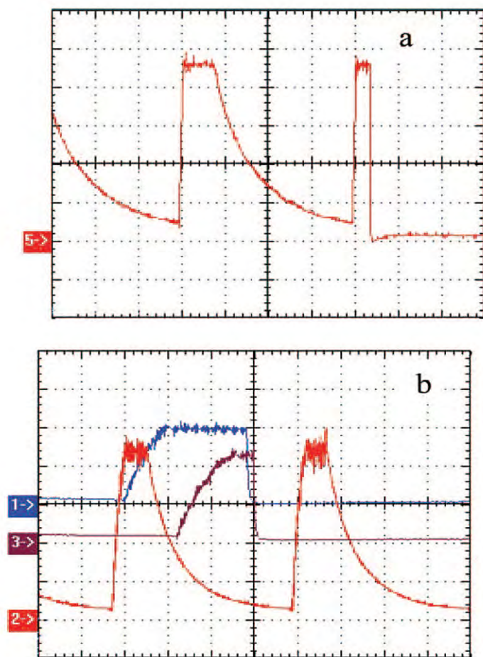
Figure 11. Typical pulse waveforms. (a) The last pulse prior to breakdown, followed by the pulse during which breakdown occurred. Gap = 7.47 mm, load = 82 MΩ, negative polarity, PRR = 50 Hz, horizontal scale = 5 ms/div, vertical scale = 30 kV/div. 5-> indicates the zero on the vertical axis. (b) Traces 1 and 3 show pulses on which breakdown occurred, with horizontal scale 0.5 ms/div, vertical scale 60 kV/div. Trace 2 shows the long trailing edge of a pulse when breakdown did not occur, horizontal scale 2 ms/div, vertical scale 30 kV/div. 1->, 2->, and 3-> show the zeros on the vertical axis for the corresponding traces. Gap = 4.94 mm, load = 20 MΩ, negative polarity, PRR=120 Hz.
