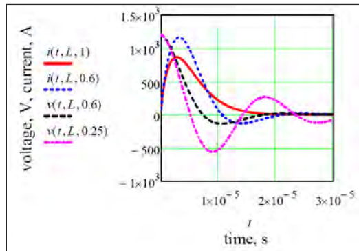
Fig. 2. Current and voltage waveforms for L=1.5\mu\text{H} ; r values (in SI) as indicated in variables' legends. r=1\Omega corresponds to critically damped discharge.
