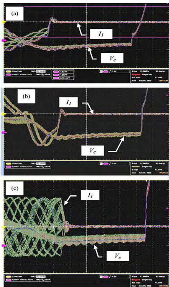
Fig. 15. Overlay of 80 frames ( V_c —100 V/div, I_1 —100 A/div) for: (a) high line, 2 kV at 1 kHz; (b) nominal line, 6 kV at 1 kHz; and (c) high line, 10 kV at 1 kHz. Horizontal axis 4 \mu s/div.
