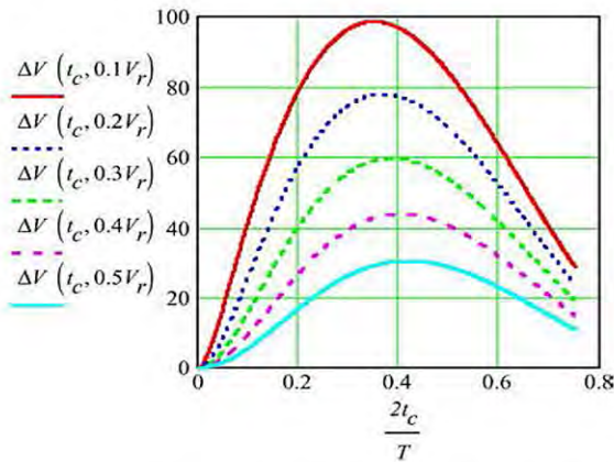
Fig. 24. Load voltage overshoot dependence on EOC timing t_c for V_r = 850\text{ V} . Load voltage in fractions of V_r serves as parameter.
