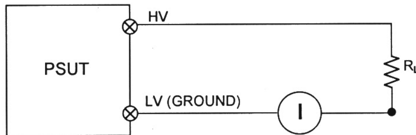
Figure 8. Current Regulation
