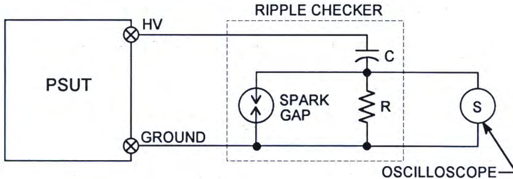
Figure 12. Ripple Measurement
