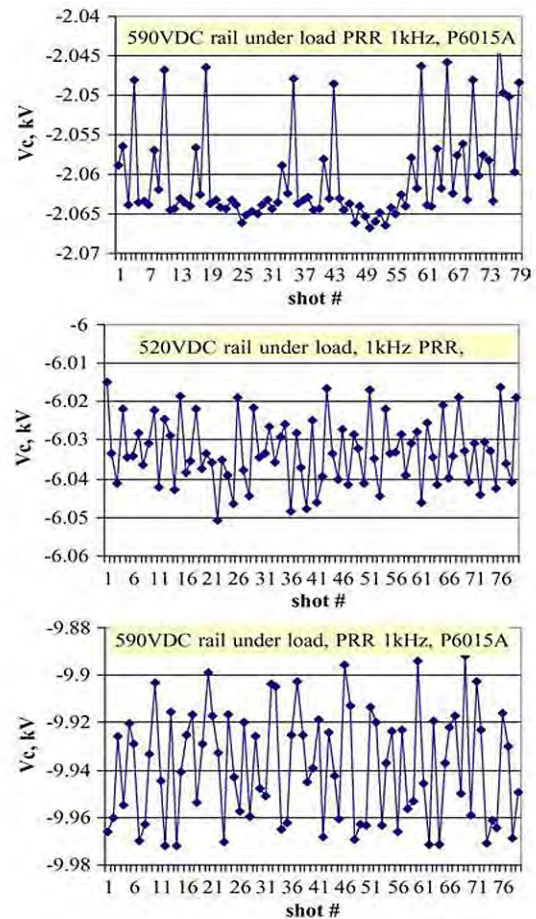
Fig. 14. Shot-to-shot variability taken with FastFrame. C_s = 420 nF, 1 kHz repute, 2-kV, 6-kV, and 10-kV settings. See inset annotations for rail voltage.
