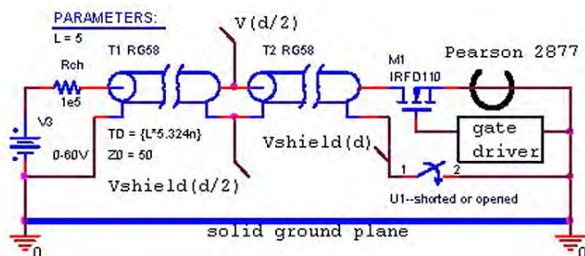
Figure 7. Experimentation scheme.
