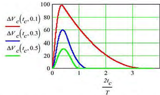
Fig. 27. Load voltage increment dependence on EOC timing t_c for V_r = 850\text{ V} . Compare to Fig. 24.
