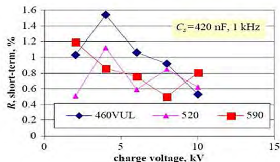
Fig. 16. Short-term repeatability.
