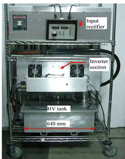
Fig. 5. Laboratory HVPS.
