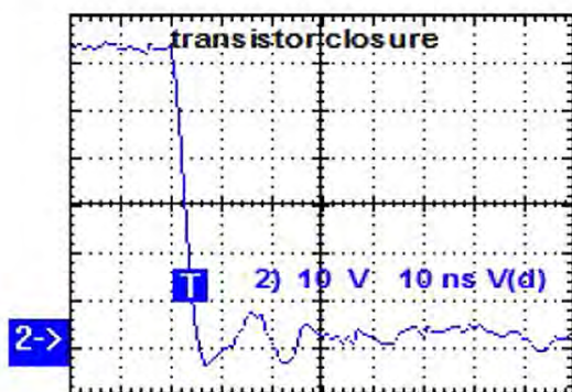
Figure 8. Transistor closure. Waveform annotation here and further gives scales' information (vertical – 10 V/div, horizontal – 10 ns/div) and legend.
