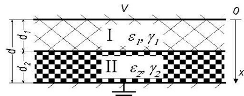
Fig. 1. Flat capacitor with two layers of non-ideal isotropic insulation.
