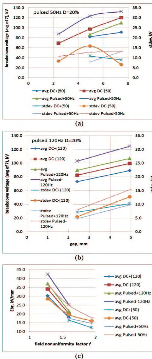
Figure 12. Test results (2011). (a) DC and pulsed test at PRR = 50 Hz, D = 20%. (b) DC and pulsed test at PRR = 120 Hz, D = 20%. (c) Dependence of the breakdown field E_{br} on field nonuniformity factor f . c is constructed using the data in a and b (note the uniformity of the data series legends in a, b, and c).
