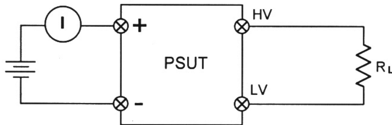
Figure 10. DC Input Current Measurement
