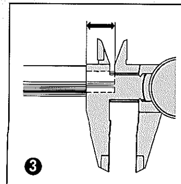
Step Measuring
