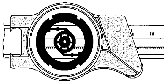
Anti-backlash pinion
