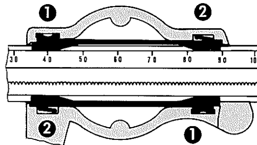
Guiding system
