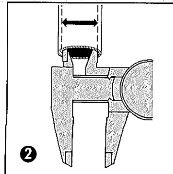
Inside Measuring
