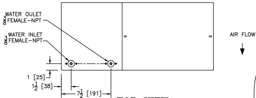
TOP VIEW
