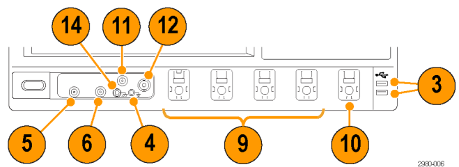
DPO70000DX Series
