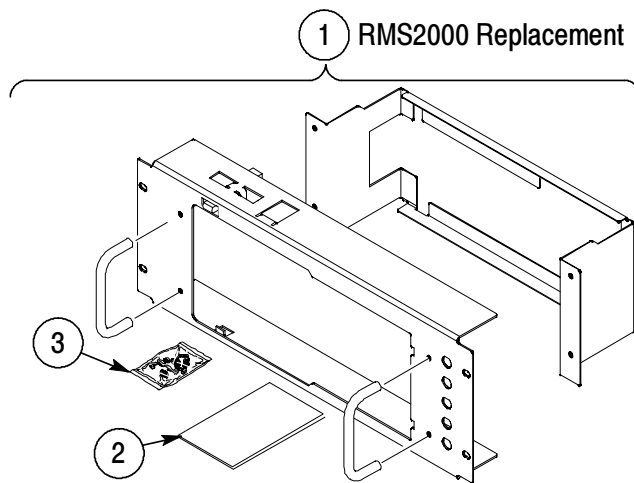
Figure 1: RM2000 Rackmount Kit parts
