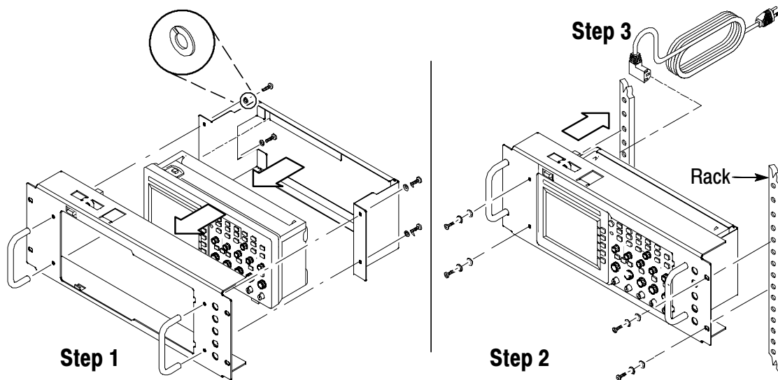
Figure 2: RM2000 Rackmount assembly
