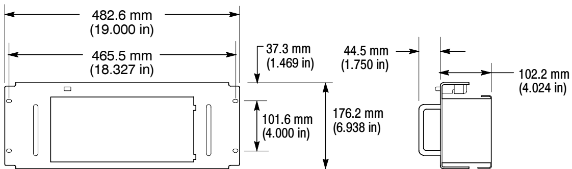
Figure 3: Dimensions of the RM2000 Rackmount
