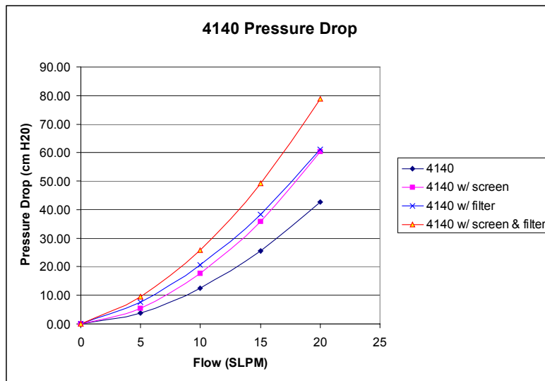
Figure A-1 Pressure Drop
