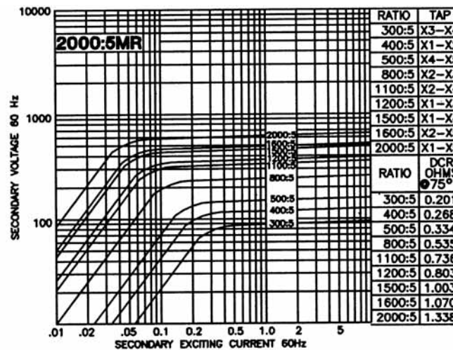
Model 143-202MR - rating C400
