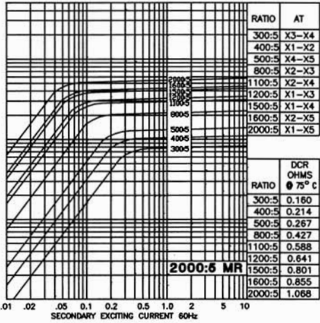
MODEL 786 - 202MR - rating C400
