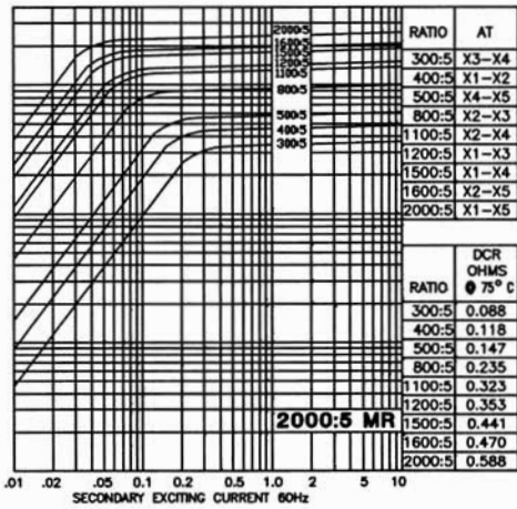
MODEL 781 - 202MR - rating C200
