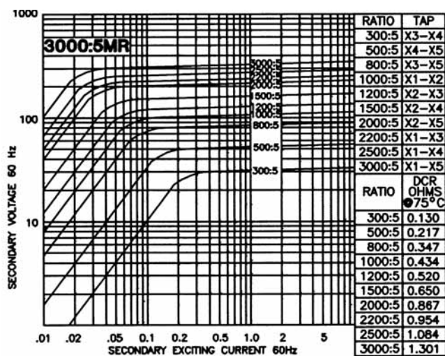
Model 135-302MR - rating C200
