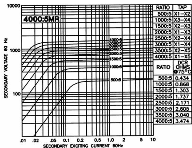
Model 145-402MR - rating C800
