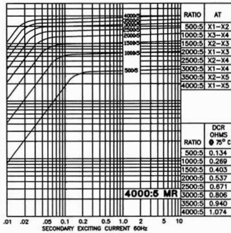
MODEL 781 - 402MR - rating C200
