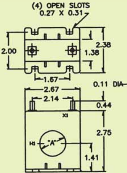
SFT Models
