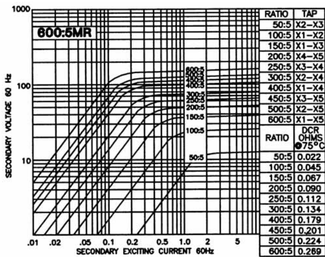
Model 139-601MR - rating C100
