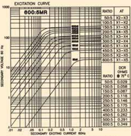
MODEL 786 - 601MR - rating C200
