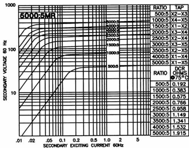
Model 140-502MR - rating C200
