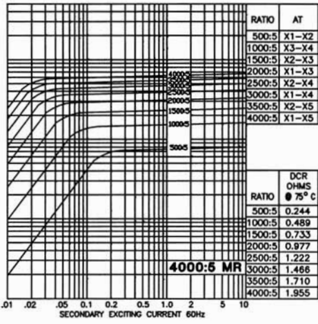
MODEL 788 - 402MR - rating C400
