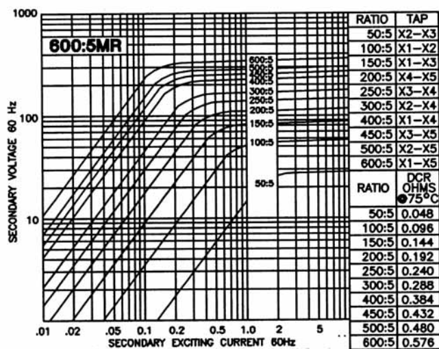
Model 145-601MR - rating C200 TRF= 2.0 ● 30°C, 1.5 ● 55°C amb.
