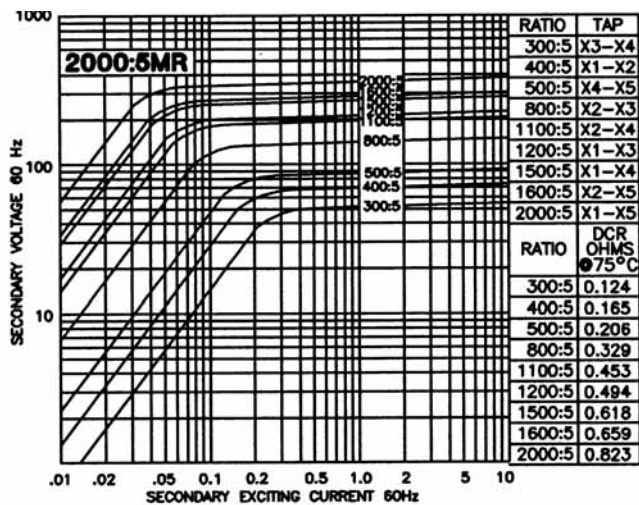
Model 139-202MR - rating C200
