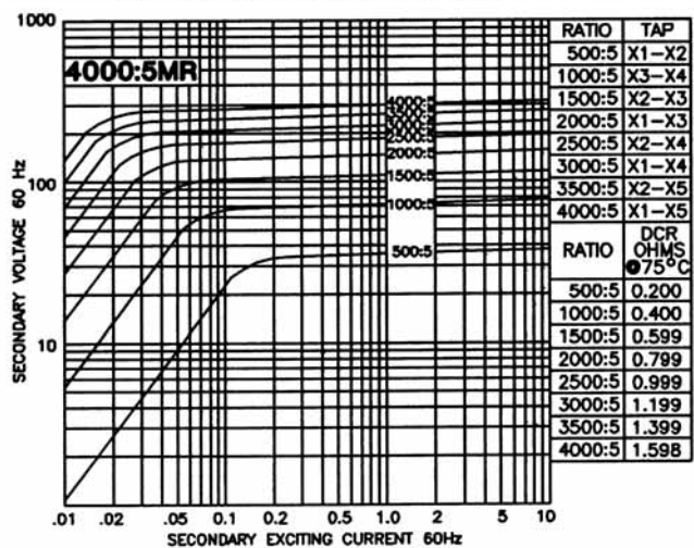
Model 135-402MR - rating C200
