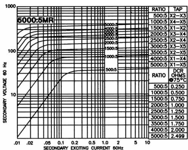
Model 135-502MR - rating C200
