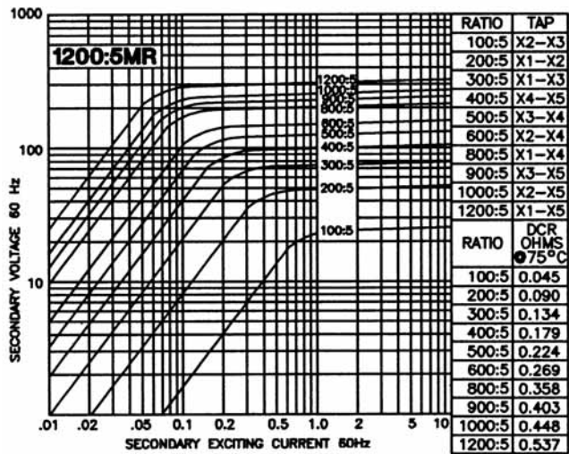
Model 139-122MR - rating C200
