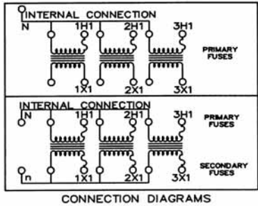
CONNECTION DIAGRAMS
