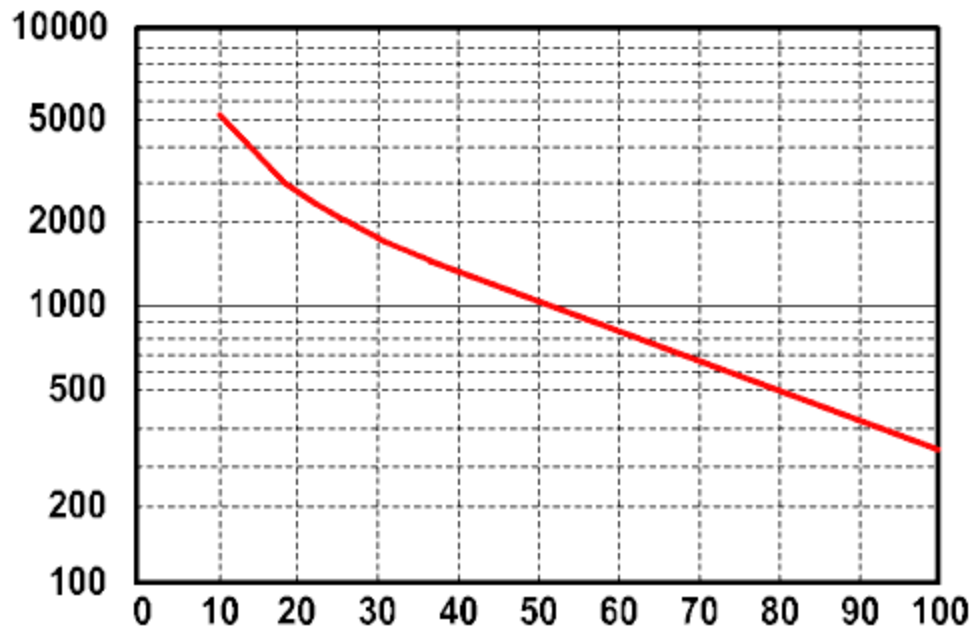
Depth-of-Discharge (DoD)
