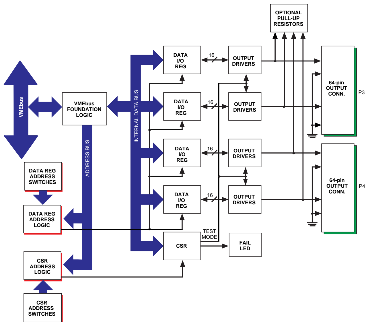
Figure 1. VMIVME-2120 Functional Block Diagram
