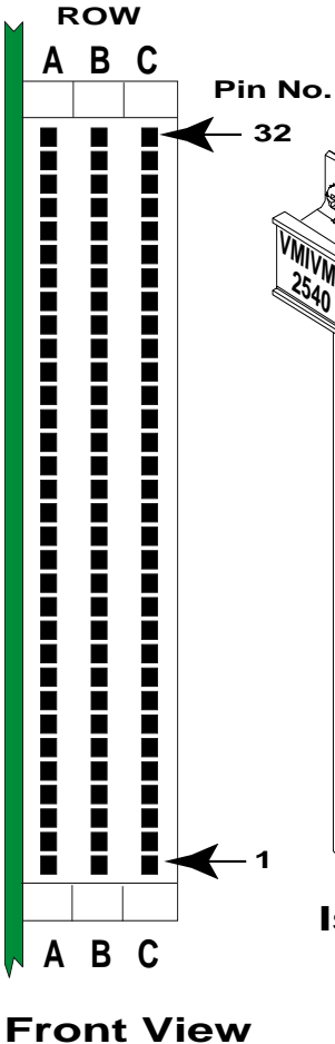
Figure 2-3 P3/P4 Pinout Layout
