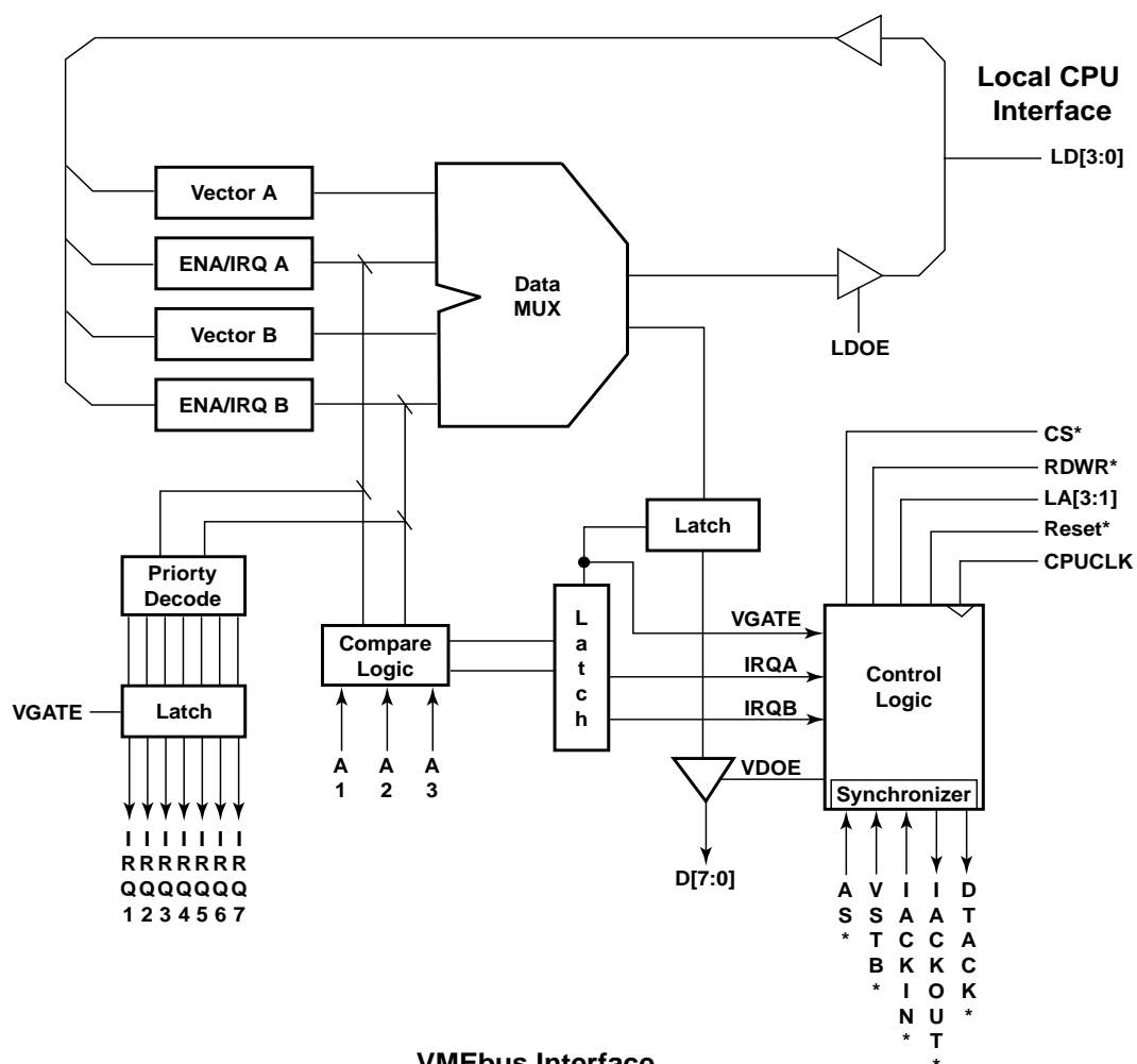
Figure 1-7 Intelligent Interface Interrupter Module
