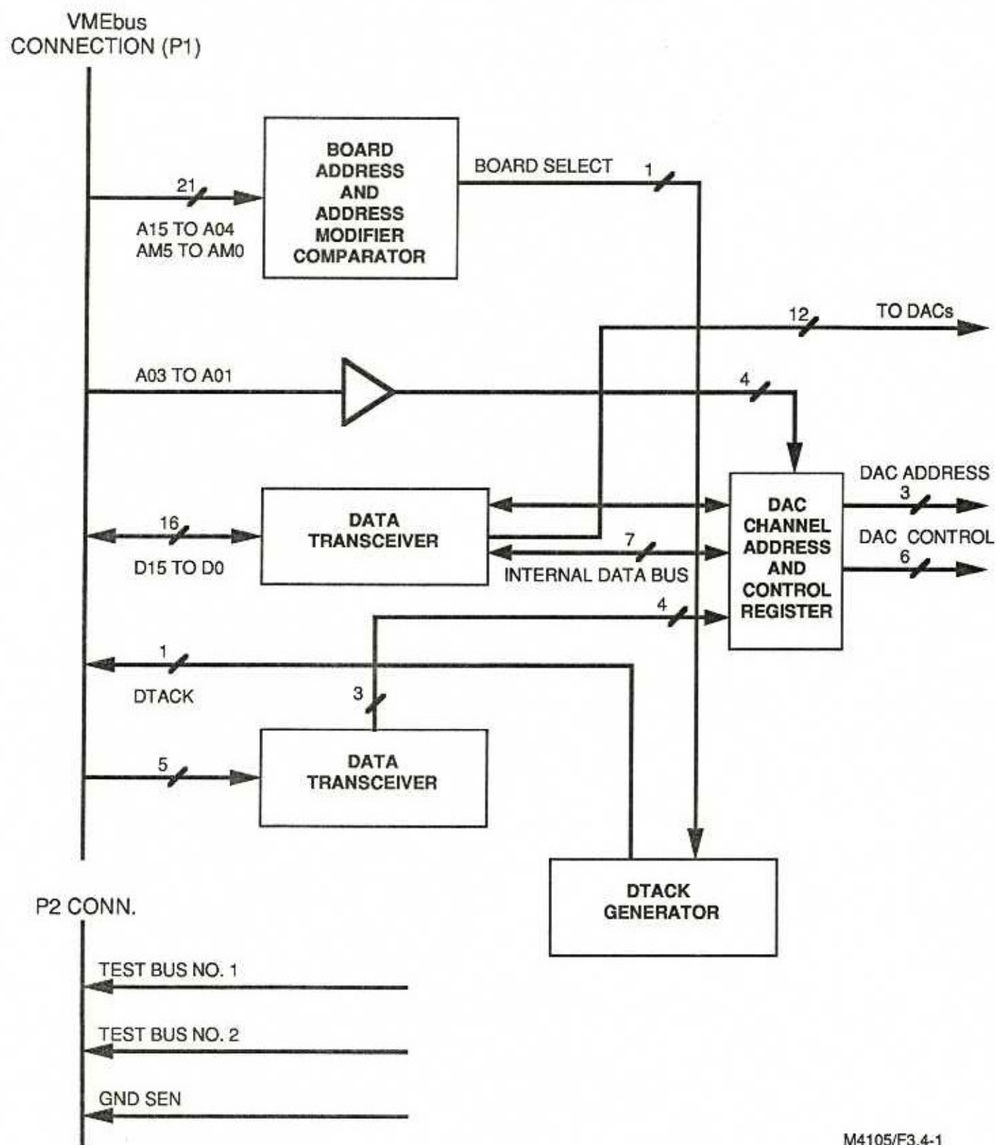
Figure 3.4-1. VMEbus Interface Logic and Interface Signals
