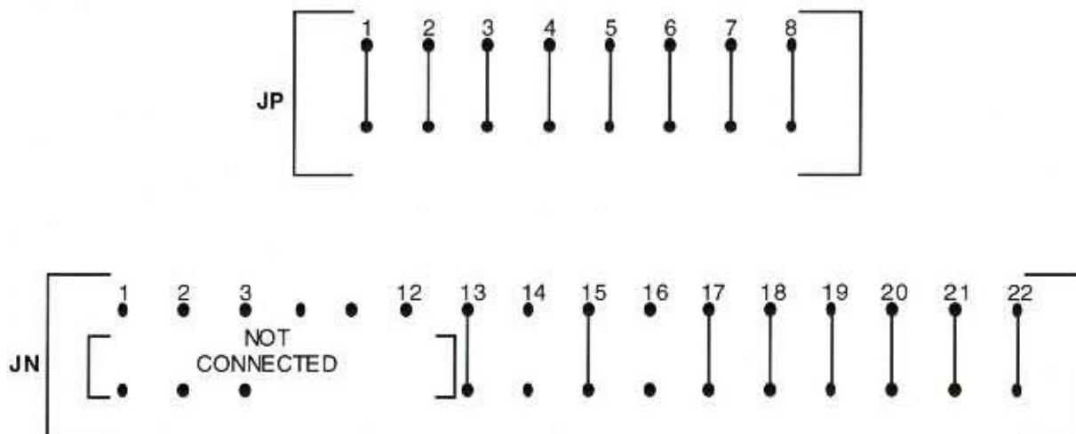
Figure 5.14-1. Jumper Configuration Analog Outputs Out P2 Connector
