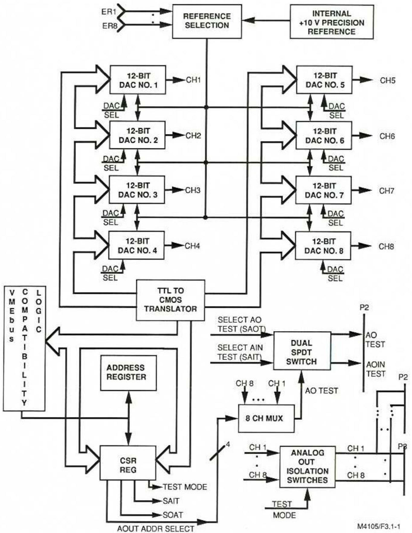
Figure 3.1-1. VMIVME-4105 Board
