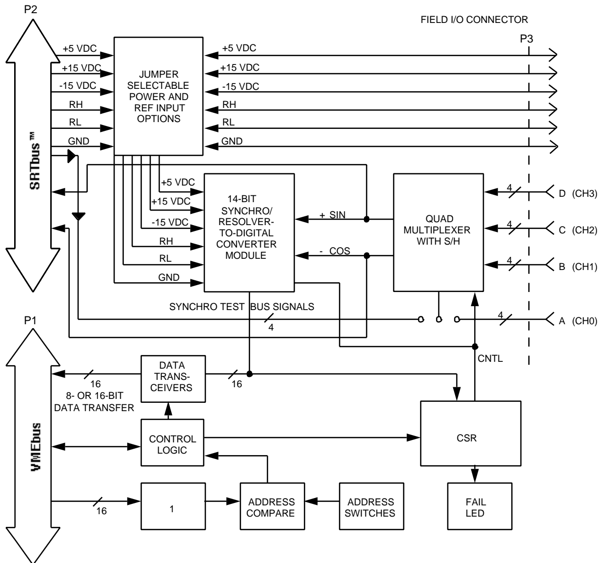
Figure 1 VMIVME-4911 Functional Block Diagram
