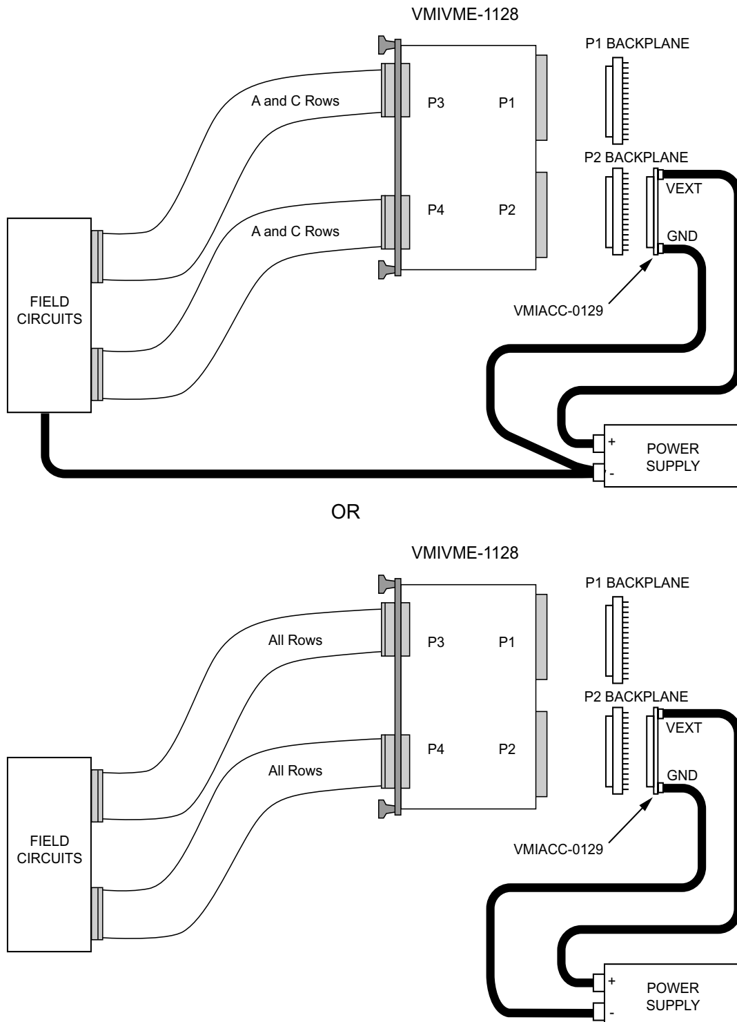
Figure 1. P2 External Power Connections
